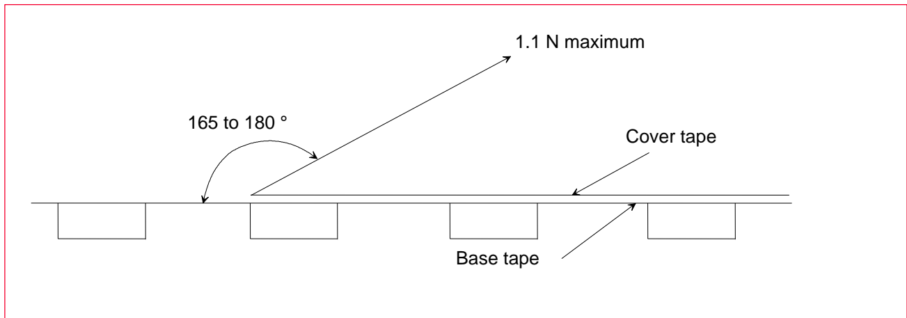
Figure 21: Peeling Force
