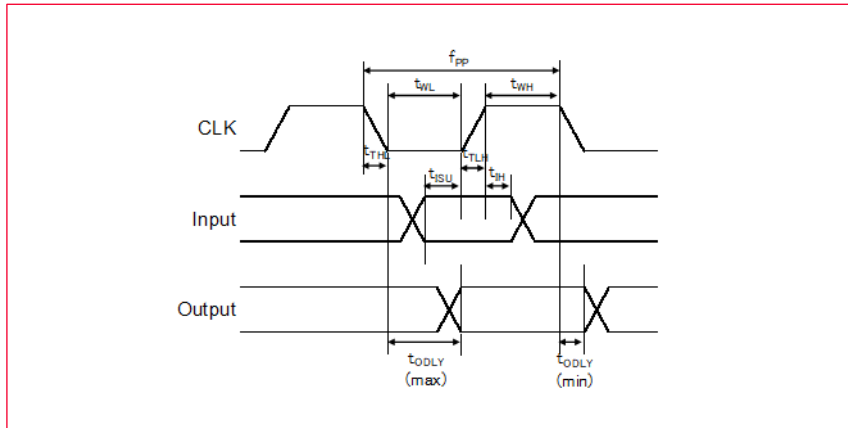
Figure 17: SDIO Protocol Timing Diagram - Default Mode
