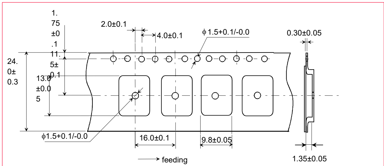
Figure 28: Dimensions of Tape (Unit: mm)
