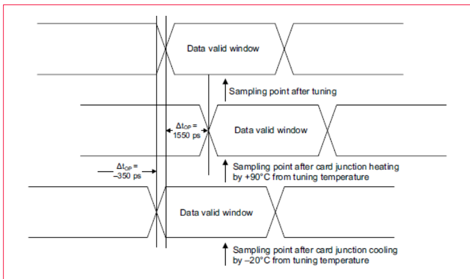
Figure 23: Δt op Consideration for Variable Data Window - SDR 104 Mode
