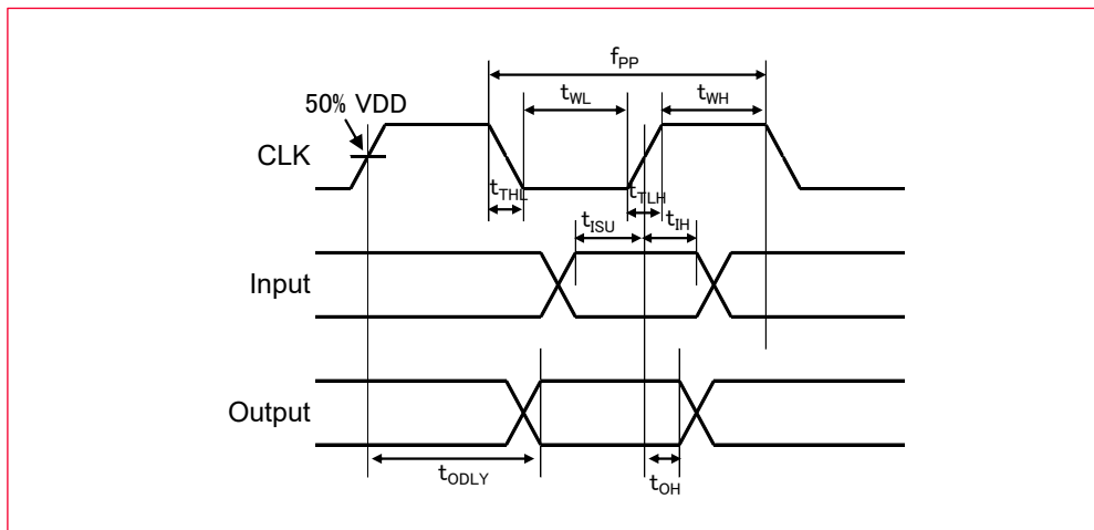
Figure 18: SDIO Protocol Timing Diagram - High-Speed Mode
