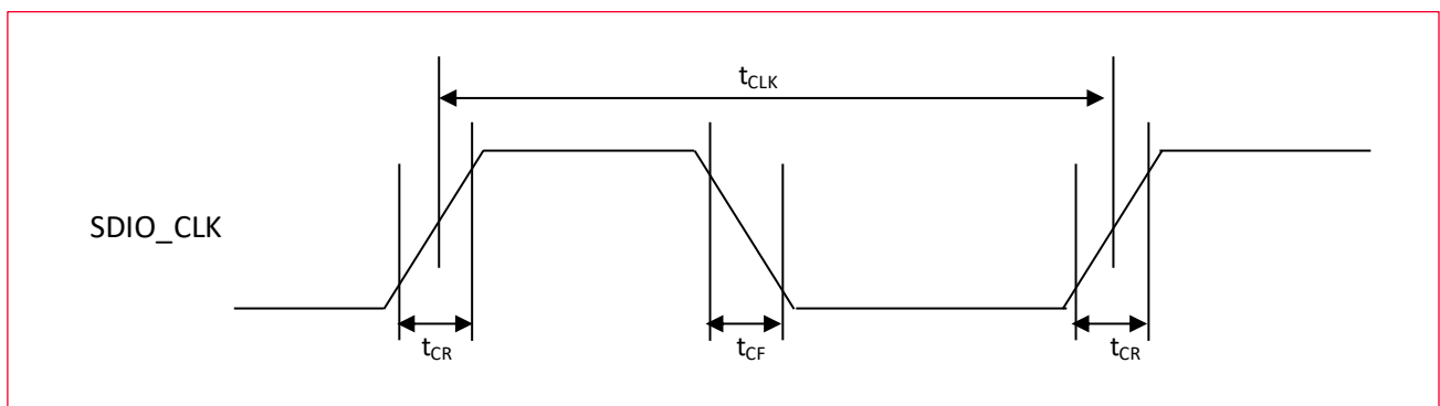
Figure 19: SDIO Clock Timing Diagram - SDR Mode
