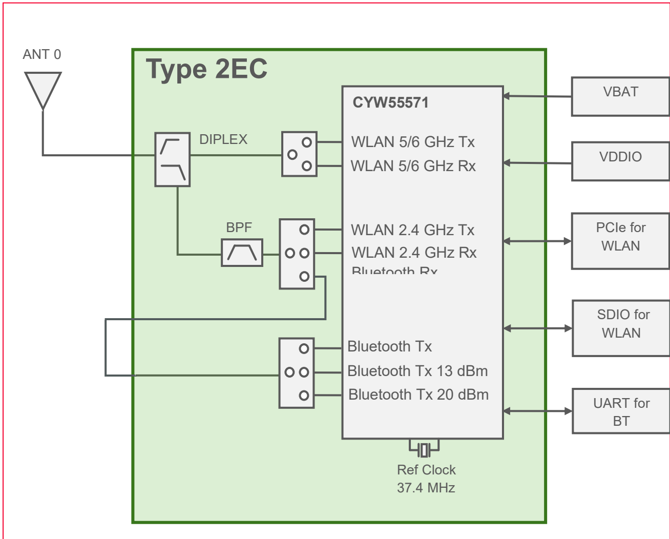
Figure 1: Block Diagram - Type 2EC for SANT Configuration
