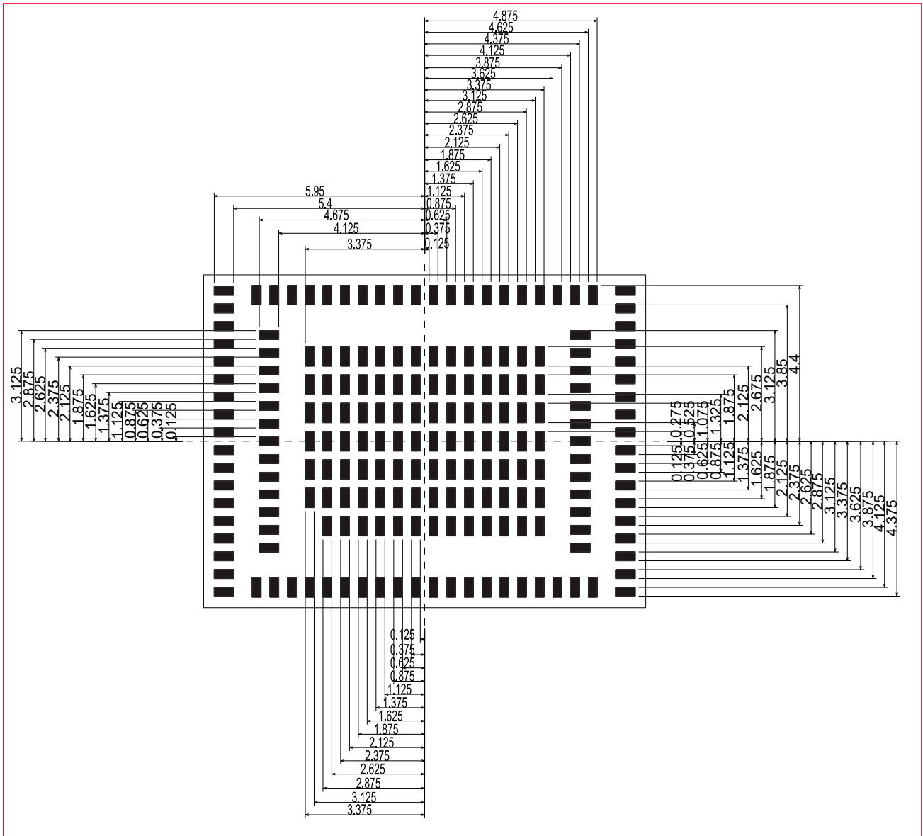
Figure 27: Land Pattern (Top View)
