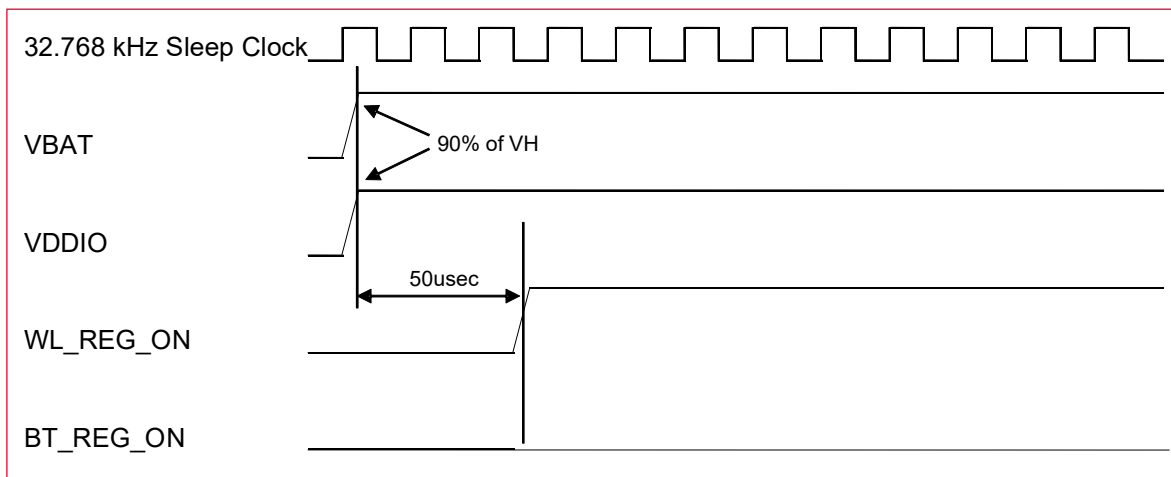
Figure 8: Power-On Sequence - WLAN ON and BT OFF
