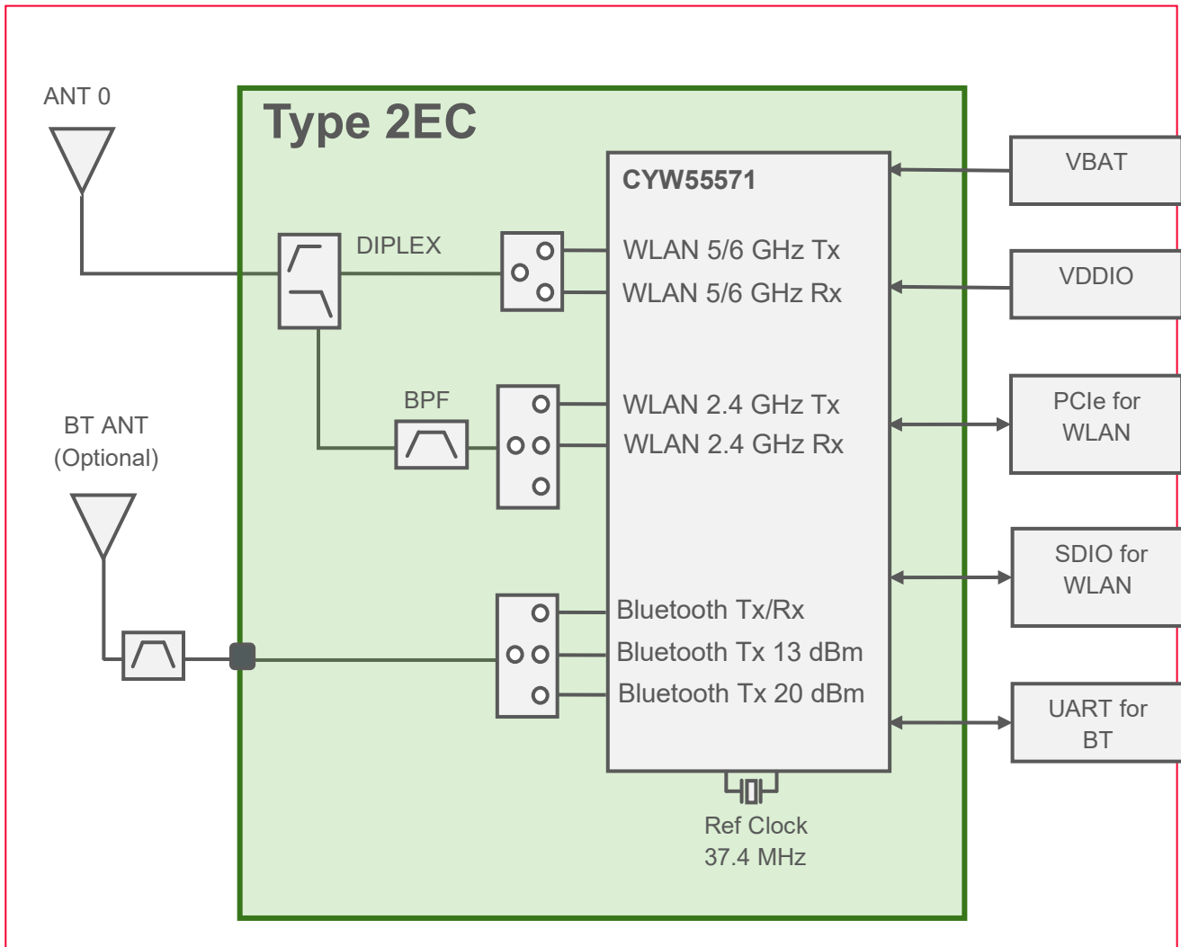
Figure 2: Block Diagram - Type 2EC for DANT Configuration
