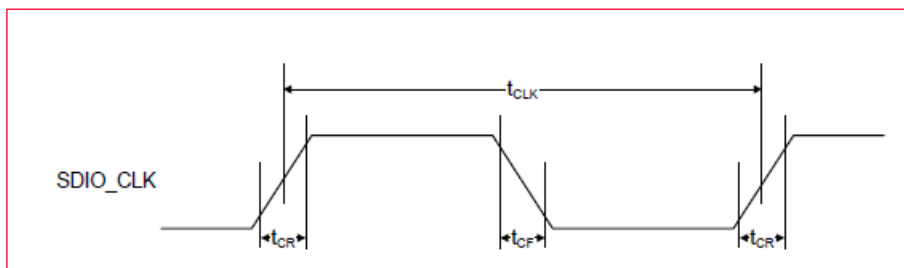
Figure 24: SDIO Clock Timing Diagram - DDR50 Mode
