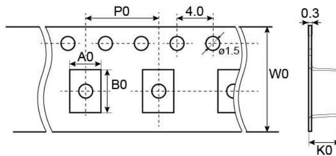
Figure 12 - Tape drawing
