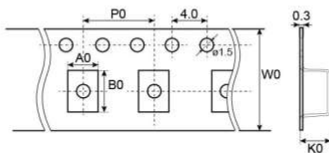
Figure 13 - Tape drawing
