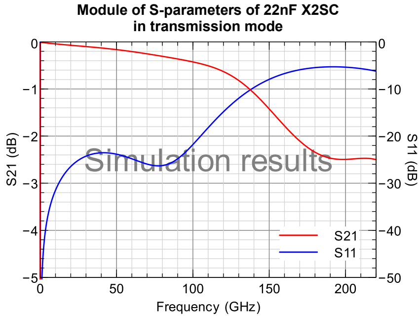
Figure 2 - 22nF X2SC simulated results (module of S-parameters)
