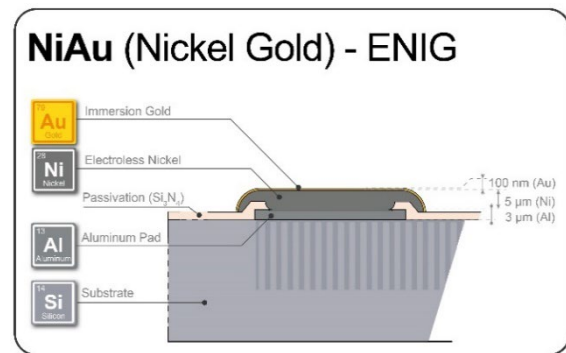
Figure 7 – Top electrode description of ENIG finishing version
