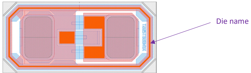
Figure 8 – Layout view
