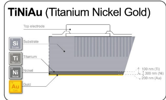
Figure 7 – Bottom electrode description
