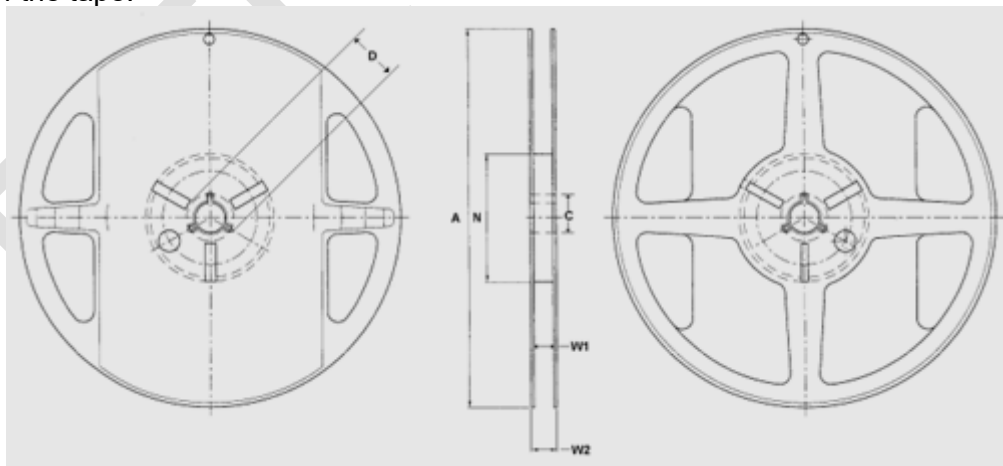
Figure 10 - Reel drawing
