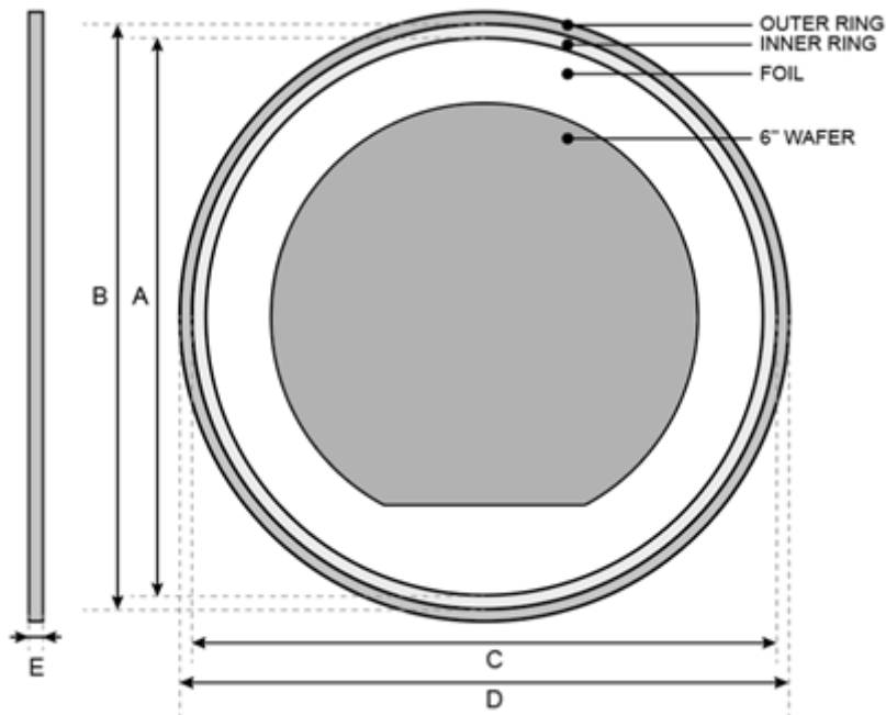
Figure 16 – Grip Ring drawing
