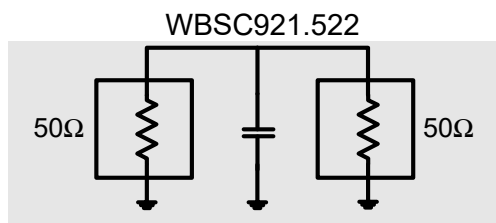
Figure 3 - 22nF WBSC/WLSC measurement schematic
