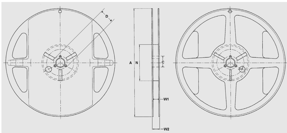
Figure 12 - Reel drawing
