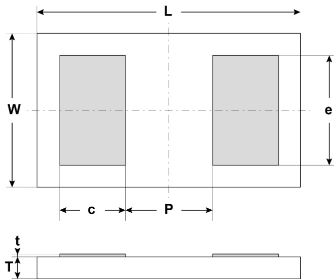
Figure 6 – Layout view
