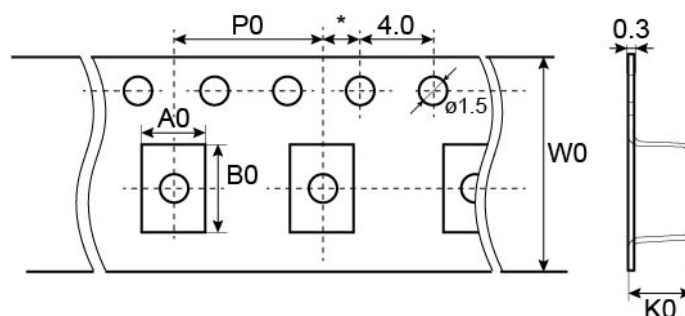
Figure 8 - Tape drawing
