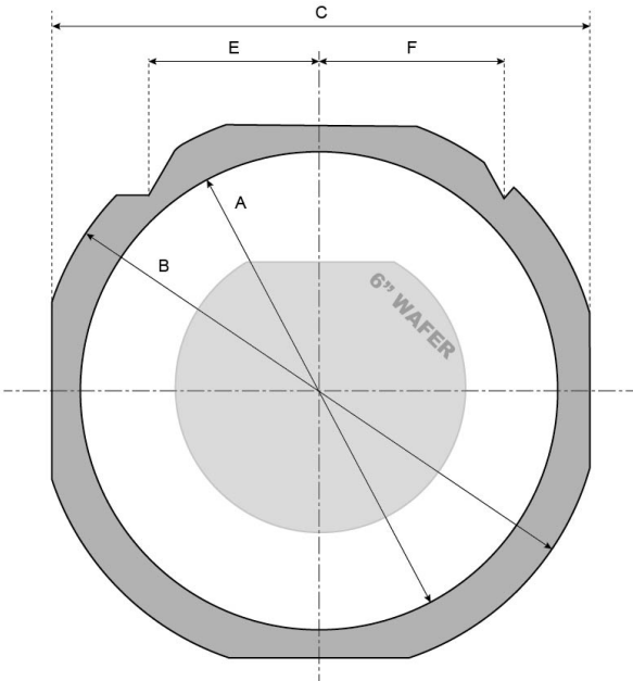
Figure 10 FF108 Frame with a 6" wafer
