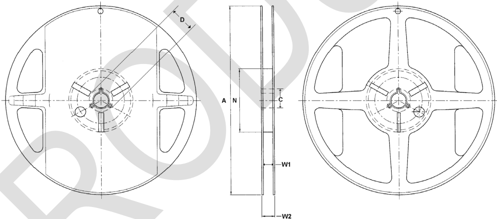
Figure 7 - Reel drawing
