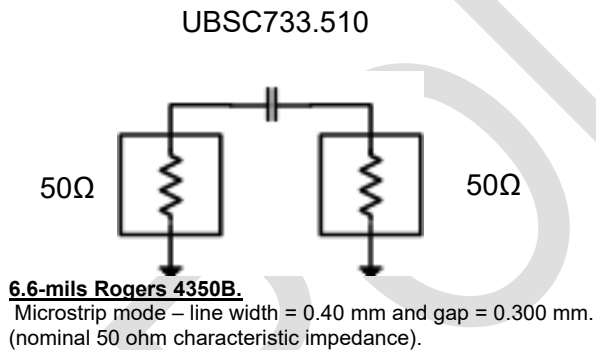
Figure 3 - 10nF UBSC measurement schematic
