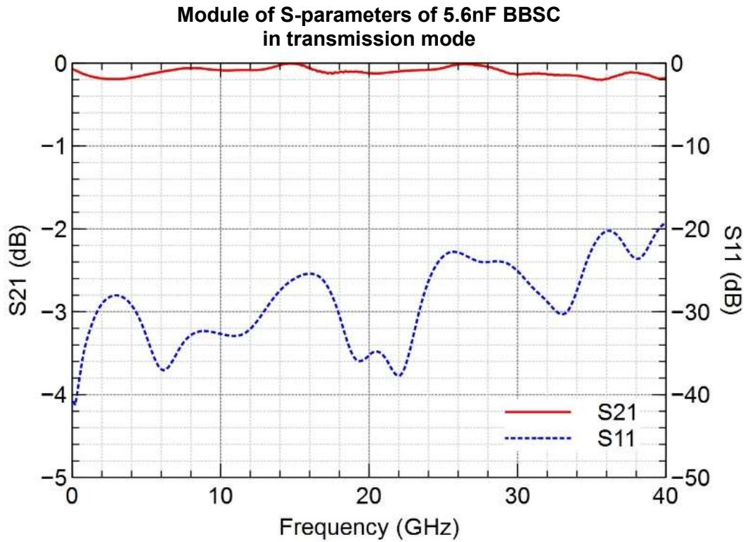
Figure 2 – 5.6nF BBSC measurement results (module of S-parameters)
