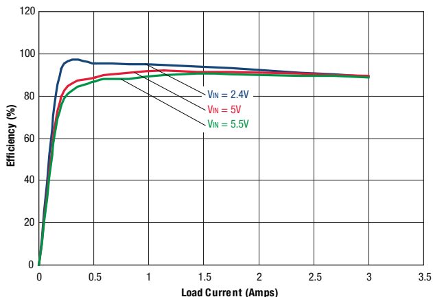
Efficiency vs. Line Voltage and Load Current @ +25°C (V OUT = 1.5V)
