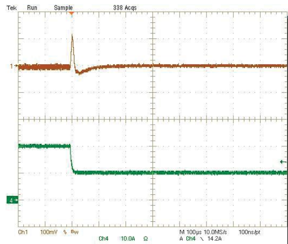
Step Load Transient Response (Vin=12V, Vout=5.0V, Cload=188uF, Iout=20 to 10A) Trace 1=Vout, 100 mV/div(AC), Trace 4=Iout, 10A/div.
