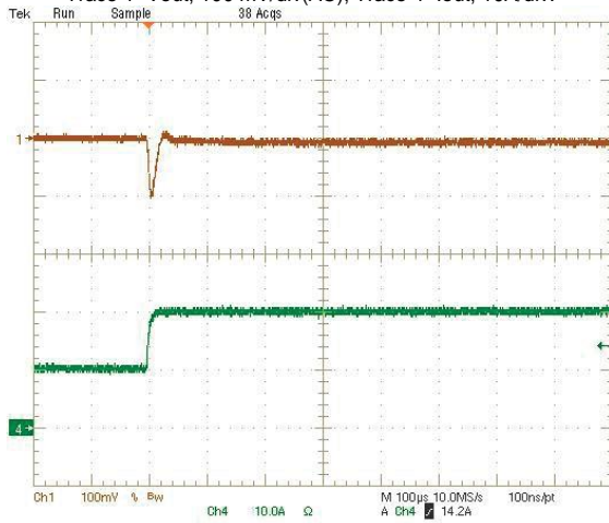
Step Load Transient Response (Vin=12V, Vout=1.2V, Cload=188uF, Iout=10 to 20A) Trace 1=Vout, 100 mV/div(AC), Trace 4=Iout, 10A/div.
