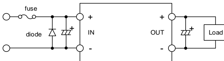
Figure11. Circuit example with a diode and fuse
