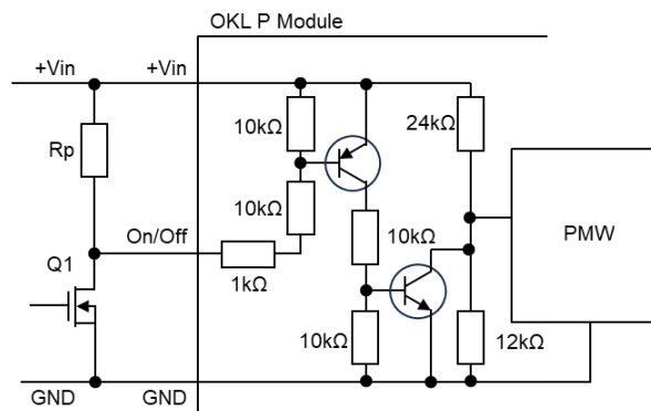
BOM → Rp → 20k BOM → Q1 → Q SMT Nch-MOS 30V
