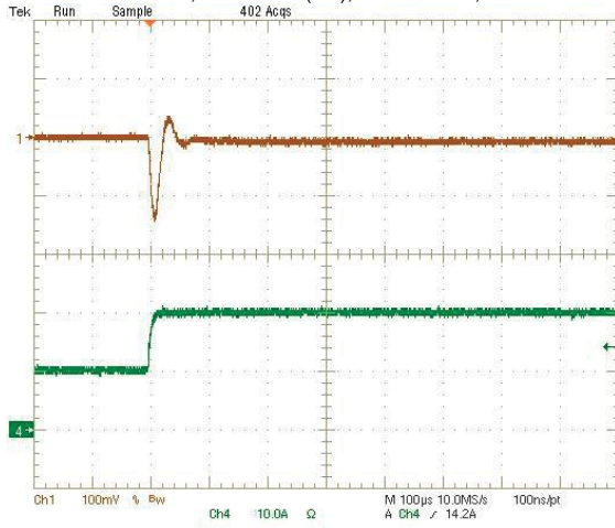
Step Load Transient Response (Vin=7V, Vout=0.69V, Cload=188uF, Iout=10 to 20A) Trace 1=Vout, 100 mV/div(AC), Trace 4=Iout, 10A/div.
