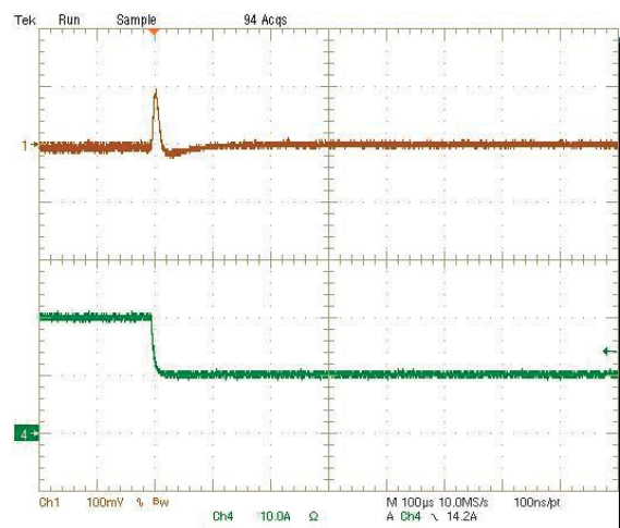
Step Load Transient Response (Vin=12V, Vout=3.3V, Cload=188uF, Iout=20 to 10A) Trace 1=Vout, 100 mV/div(AC), Trace 4=Iout, 10A/div.
