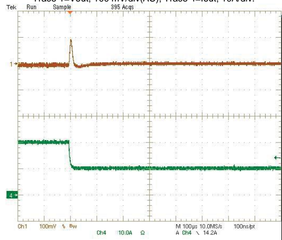
Step Load Transient Response (Vin=12V, Vout=2.5V, Cload=188uF, Iout=20 to 10A) Trace 1=Vout, 100 mV/div(AC), Trace 4=Iout, 10A/div.
