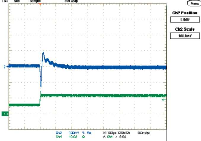
Step Load Transient Response (Vin=12V, Vout=1.8V, Cload=188uF, Iout=6 to 12A) Trace 2=Vout, 100 mV/div, Trace 4=Iout, 10A/div.
