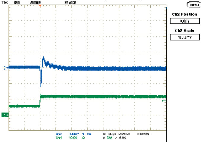
Step Load Transient Response (Vin=12V, Vout=2.5V, Load=188μF, Iout=6A to 12A) Trace 2=Vout, 100 mV/div, Trace 4=Iout, 10A/div.
