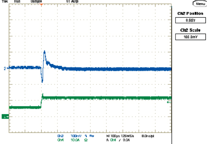
Step Load Transient Response (Vin=12V, Vout=1.2V, Cload=188uF, Iout=6 to 12A) Trace 2=Vout, 100 mV/div, Trace 4=Iout, 10A/div.
