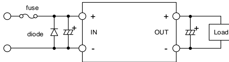
Figure 12. Circuit example with a diode and fuse
