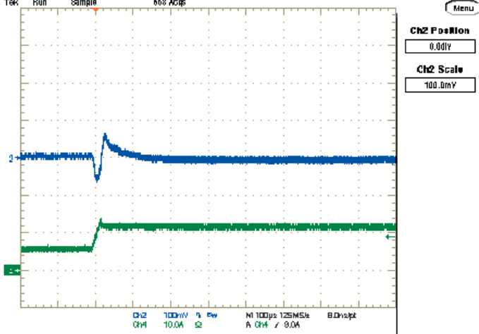
Step Load Transient Response (Vin=7V, Vout=0.69V, Cload=188uF, Iout=6 to 12A) Trace 2=Vout, 100 mV/div, Trace 4=Iout, 10A/div.
