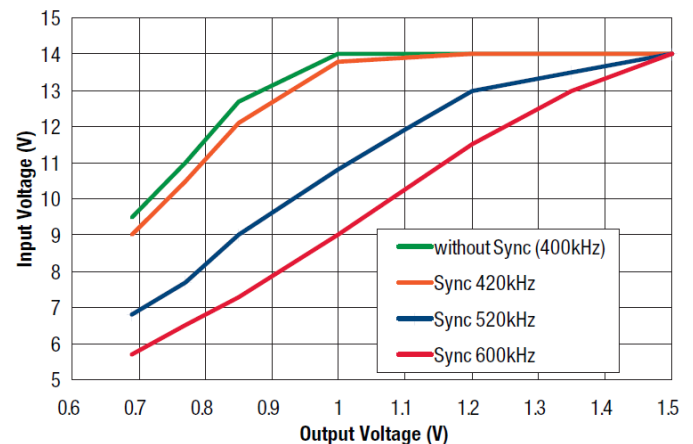
Figure 10. Voltage Range Graph (range expansion)
