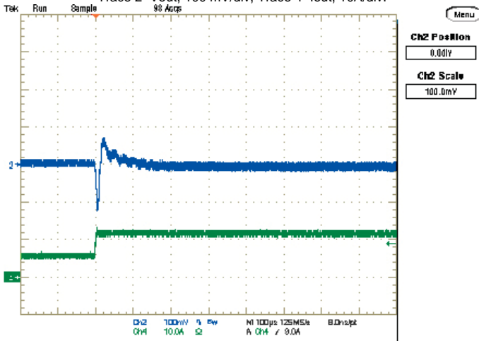
Step Load Transient Response (Vin=12V, Vout=2.5V, Cload=188uF, Iout=6 to 12A) Trace 2=Vout, 100 mV/div, Trace 4=Iout, 10A/div.
