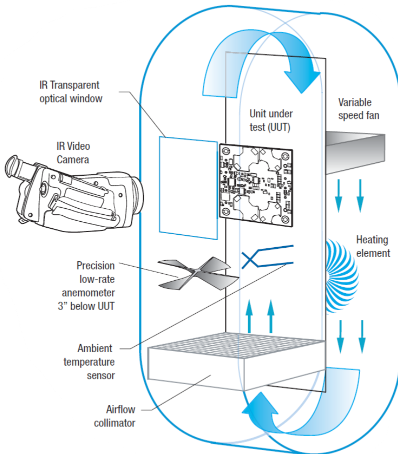
Figure 11. Vertical Wind Tunnel
