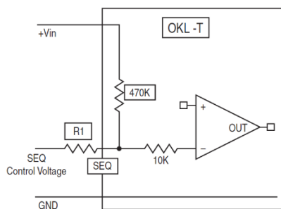
Figure 6. Sequencing Signal Interface of Module
