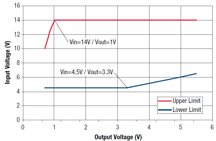
Figure 9. Voltage Range Graph
