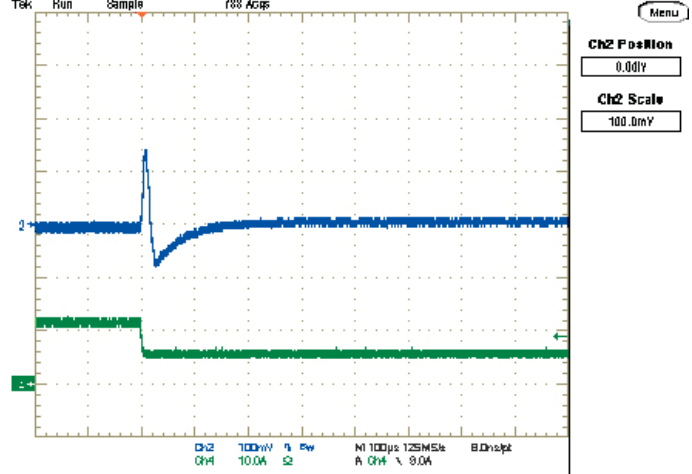
Step Load Transient Response (Vin=12V, Vout=1.2V, Cload=188uF, Iout=12 to 6A) Trace 2=Vout, 100 mV/div, Trace 4=Iout, 10A/div.
