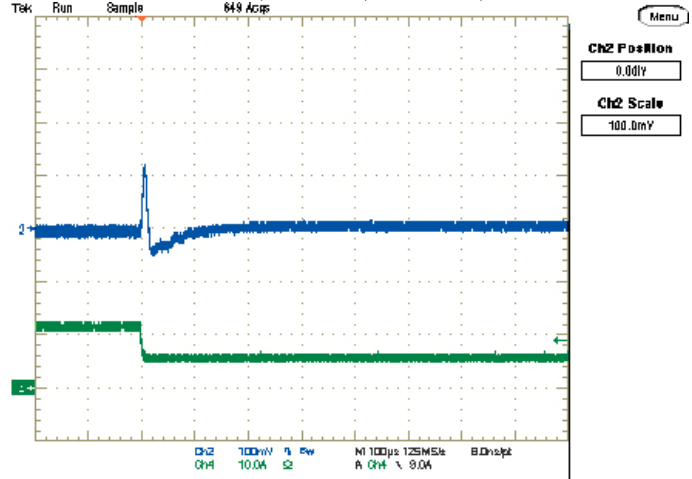
Step Load Transient Response (Vin=12V, Vout=2.5V, Load=188μF, Iout=12A to 6A) Trace 2=Vout, 100 mV/div, Trace 4=Iout, 10A/div
