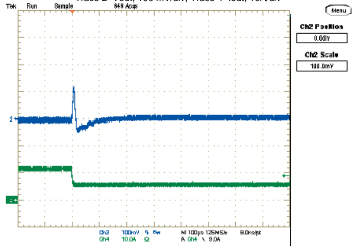
Step Load Transient Response (Vin=12V, Vout=2.5V, Cload=188uF, Iout=12 to 6A) Trace 2=Vout, 100 mV/div, Trace 4=Iout, 10A/div
