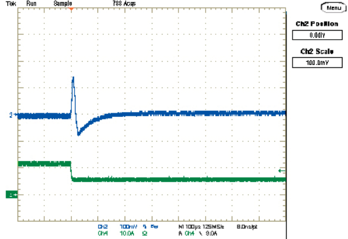
Step Load Transient Response (Vin=12V, Vout=1.2V, Load=188μF, Iout=12A to 6A) Trace 2=Vout, 100 mV/div, Trace 4=Iout, 10A/div.
