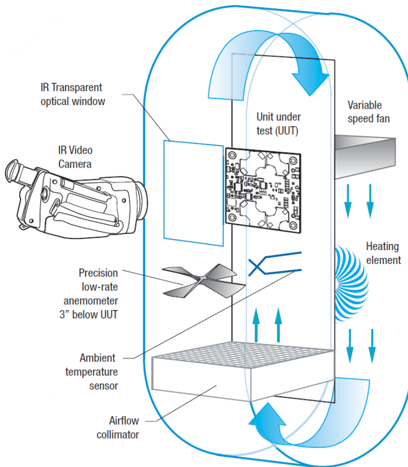
Figure 10. Vertical Wind Tunnel
