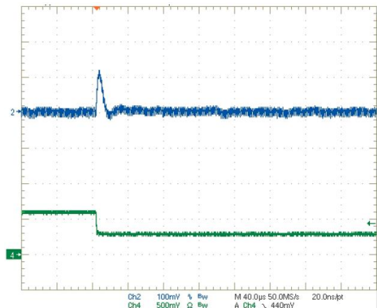
Step Load Transient Response (Vin = 12V, Vout = 1.2V, Cload = 0, Iout = 3 to 1.5A) Trace 2 = Vout, 100 mV/div. Trace 4 = Iout, 2.5A/div.
