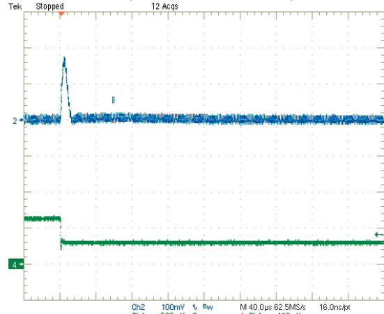
Step Load Transient Response (Vin = 5V, Vout = 3.3V, Cload = 0, Iout = 3 to 1.5A) Trace 2 = Vout, 100 mV/div. Trace 4 = Iout, 2.5A/div.
