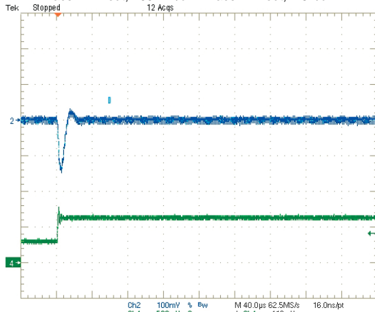
Step Load Transient Response (Vin = 5V, Vout = 1.2V, Clload = 0, Iout = 1.5 to 3A) Trace 2 = Vout, 100 mV/div. Trace 4 = Iout, 2.5A/div.
