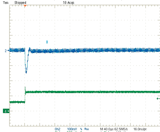
Step Load Transient Response (Vin = 5V, Vout = 3.3V, Cload = 0, Iout = 1.5 to 3A) Trace 2 = Vout, 100 mV/div. Trace 4 = Iout, 2.5A/div.
