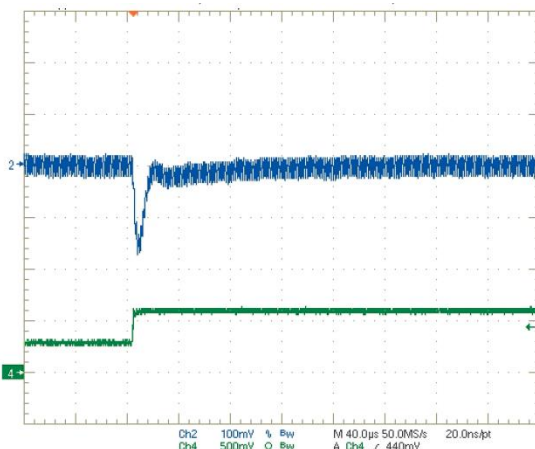
Step Load Transient Response (Vin = 12V, Vout = 2.5V, Cload = 0, Iout = 1.5 to 3A) Trace 2 = Vout, 100 mV/div. Trace 4 = Iout, 2.5A/div.
