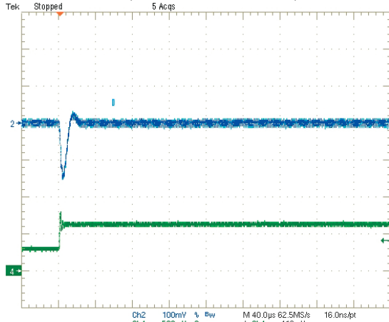
Step Load Transient Response (Vin = 5V, Vout = 1.5V, Clload = 0, Iout = 1.5 to 3A) Trace 2 = Vout, 100 mV/div. Trace 4 = Iout, 2.5A/div.
