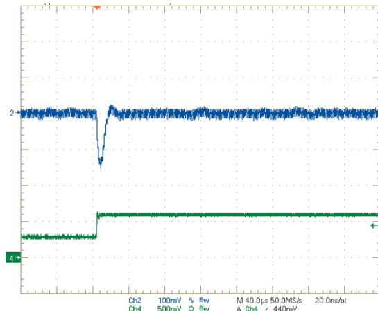
Step Load Transient Response (Vin = 12V, Vout = 1.2V, Cload = 0, Iout = 1.5 to 3A) Trace 2 = Vout, 100 mV/div. Trace 4 = Iout, 2.5A/div.
