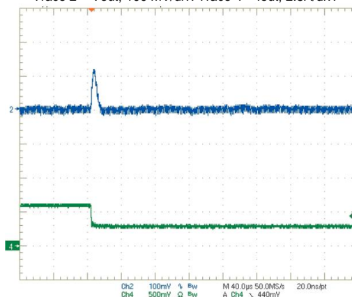
Step Load Transient Response ( V_{in} = 12V , V_{out} = 1.0V , C_{load} = 0 , I_{out} = 3 to 1.5A ) Trace 2 = V_{out} , 100 mV/div. Trace 4 = I_{out} , 2.5A/div.
