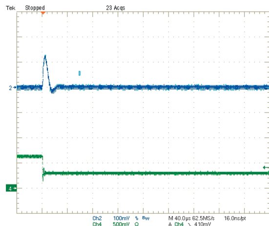
Step Load Transient Response (Vin = 5V, Vout = 1.0V, Cload = 0, Iout = 3 to 1.5A) Trace 2 = Vout, 100 mV/div. Trace 4 = Iout, 2.5A/div.
