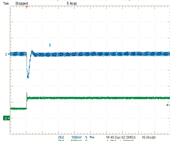
Step Load Transient Response (Vin = 5V, Vout = 2.5V, Clload = 0, Iout = 1.5 to 3A) Trace 2 = Vout, 100 mV/div. Trace 4 = Iout, 2.5A/div.
