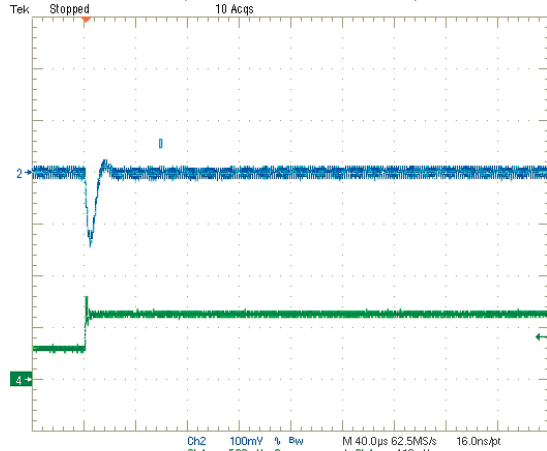
Step Load Transient Response (Vin = 5V, Vout = 1.8V, Clload = 0, Iout = 1.5 to 3A) Trace 2 = Vout, 100 mV/div. Trace 4 = Iout, 2.5A/div.
