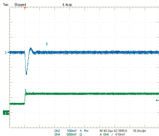
Step Load Transient Response (Vin = 5V, Vout = 1.0V, Cload = 0, Iout = 1.5 to 3A) Trace 2 = Vout, 100 mV/div. Trace 4 = Iout, 2.5A/div.
