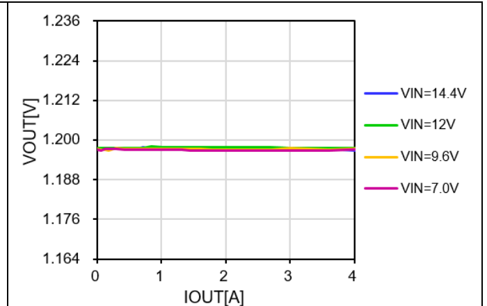
Figure 24. V OUT vs. Load Current and Line Voltage
