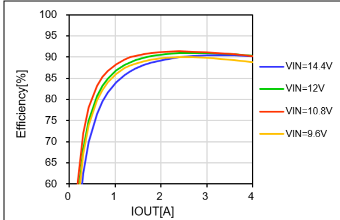
Figure 17. Efficiency vs. Load Current and Line Voltage
