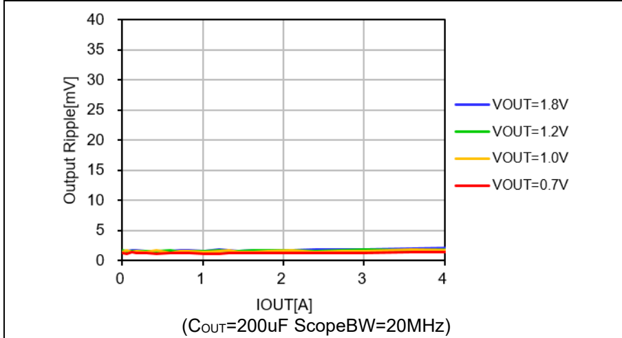
Figure 6. Output Ripple vs. Load Current and Output Voltage ( C_{OUT}=200\mu F ScopeBW=20MHz)
