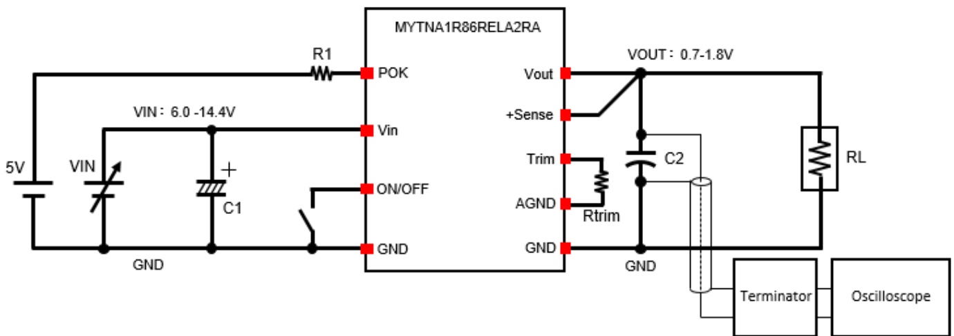
Figure 29. Test Circuit
