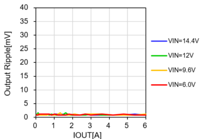
( C_{OUT} = 200\mu F , ScopeBW = 20MHz) Figure 26. Output Ripple and Noise
