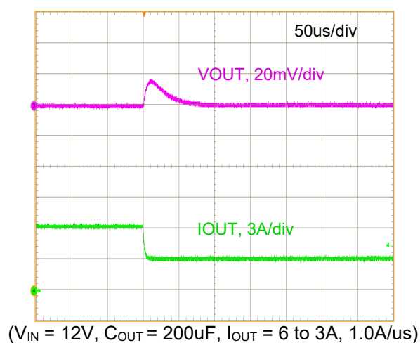
Figure 28. Step Load Transient Response
