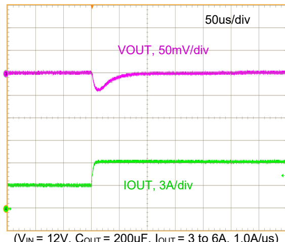
Figure 15. Step Load Transient Response
