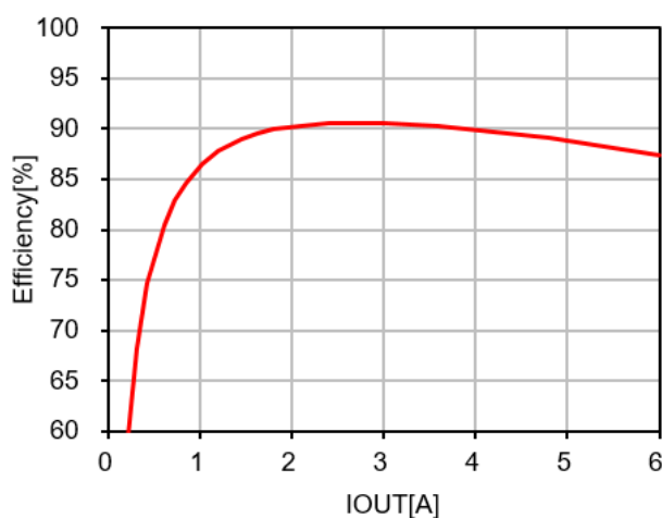
Figure 1. Efficiency Plot
