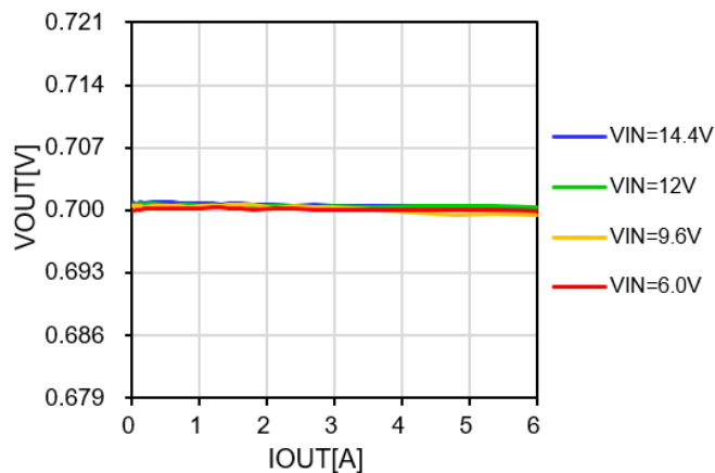
Figure 24. V_{OUT} vs. Load Current and Line Voltage
