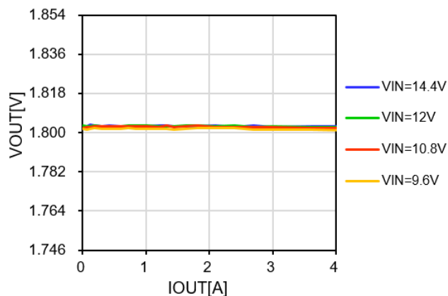
Figure 12. V OUT vs. Load Current and Line Voltage
