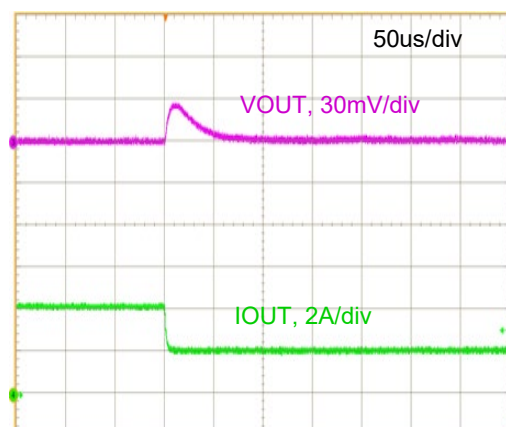
Figure 16. Step Load Transient Response
