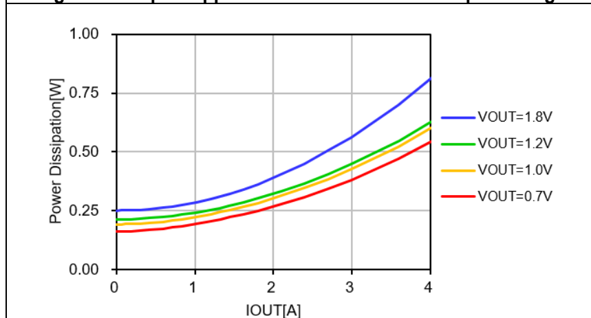
Figure 7. Power Dissipation vs. Load Current and Output Voltage
