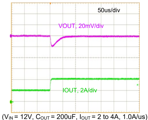
Figure 21. Step Load Transient Response
