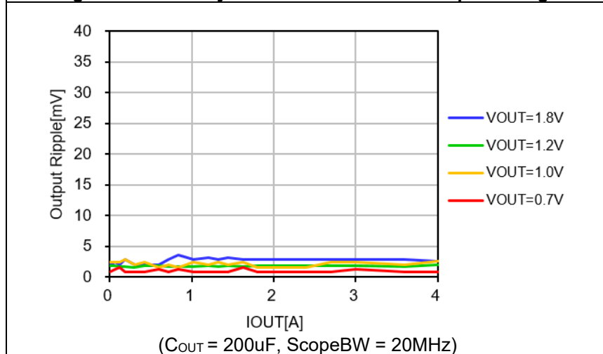
Figure 6. Output Ripple vs. Load Current and Output Voltage
