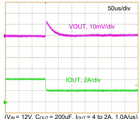
Figure 28. Step Load Transient Response
