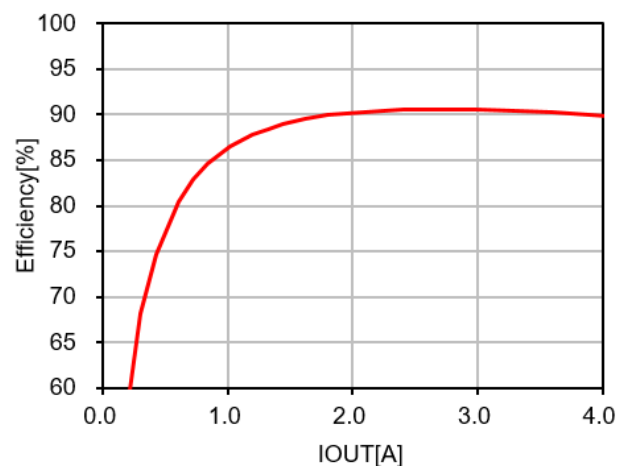
Figure 1. Efficiency Plot
