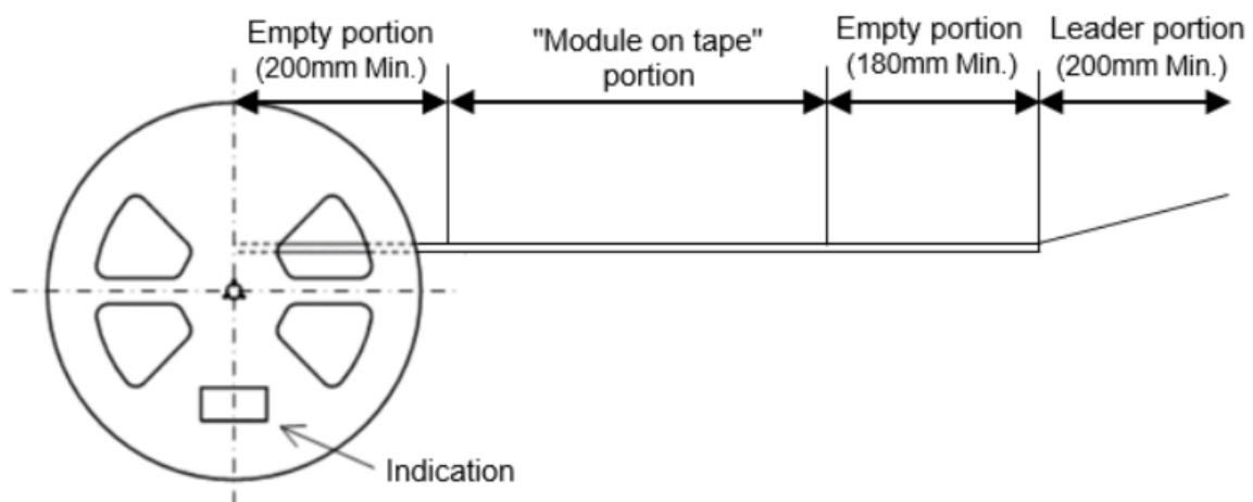
Figure 39. Taping Specification
