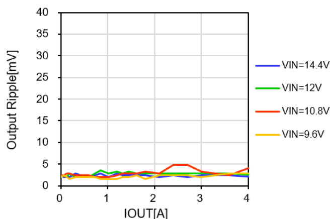
Figure 14. Output Ripple and Noise
