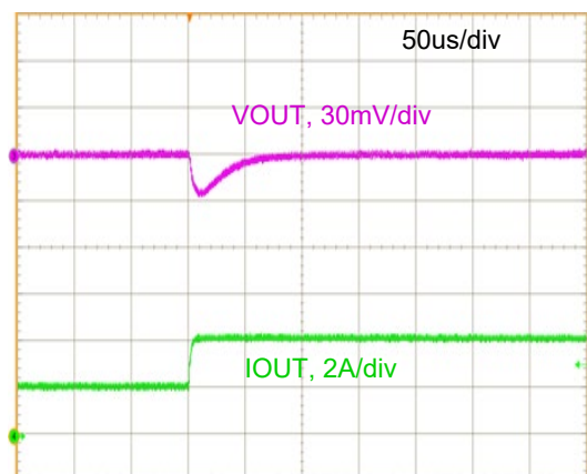
Figure 15. Step Load Transient Response
