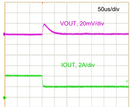
Figure 22. Step Load Transient Response
