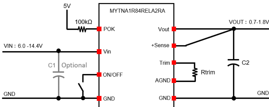
Figure 33. Application Schematic
