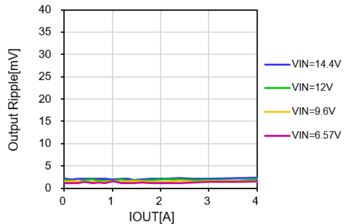
Figure 20. Output Ripple and Noise ( C_{OUT} = 200\mu F , ScopeBW = 20MHz)
