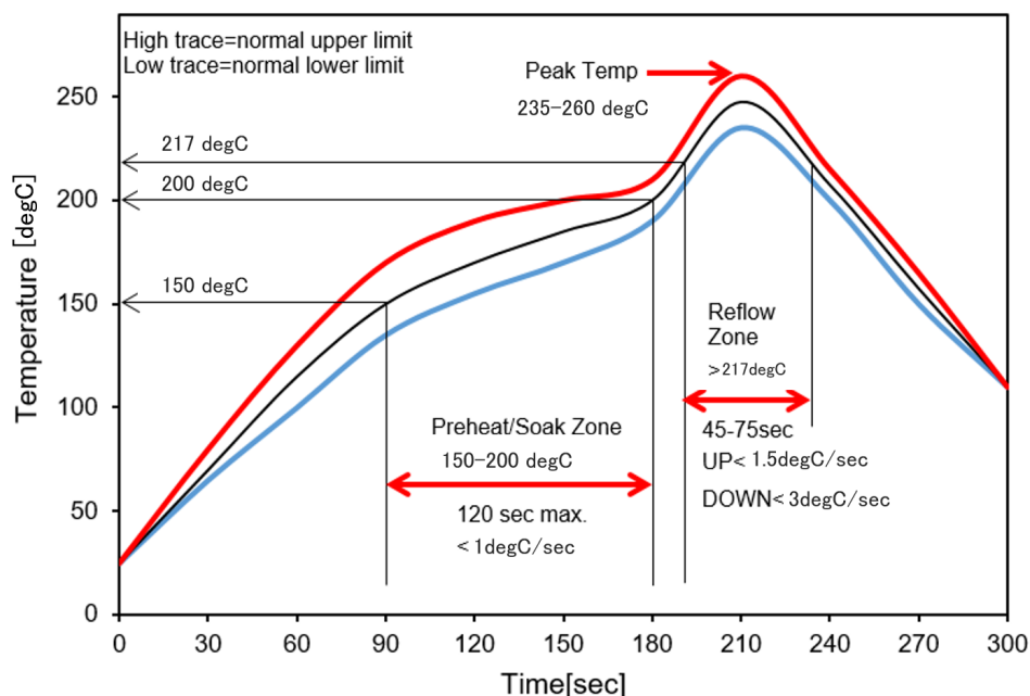
Figure 10. Reflow Profile for Sn/Ag/Cu Solder
