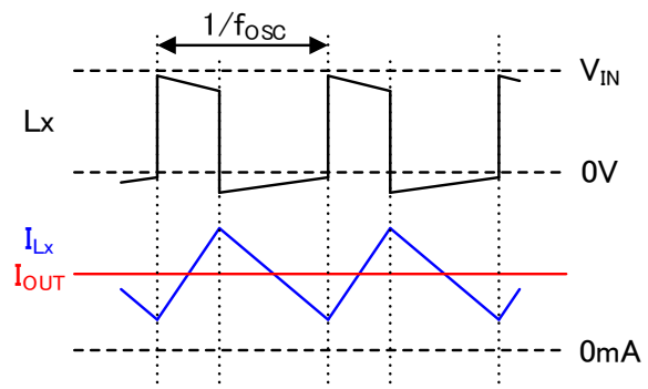
MYRGC075060B31RB (PWM/PFM control) : Example of heavy load operation
