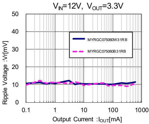
(3) Ripple Voltage vs. Output Current (MYRGC075060W31RB / MYRGC075060B31RB)
