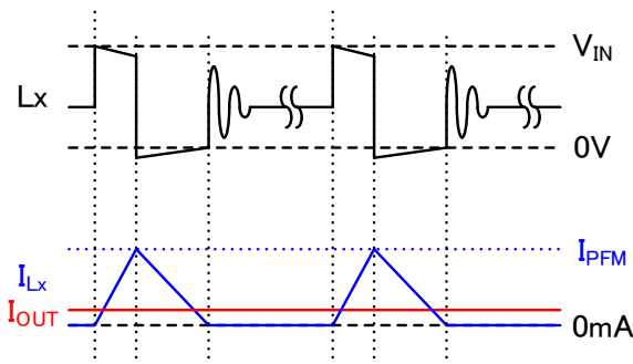
MYRGC075060B31RB (PWM/PFM control) : Example of light load operation
