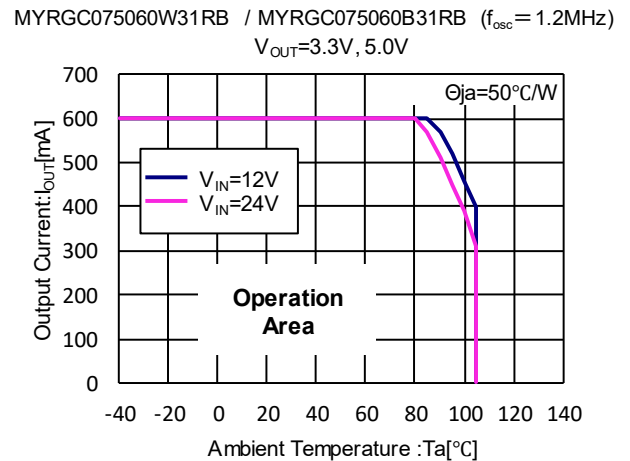
(13) Output Current Operation Area
