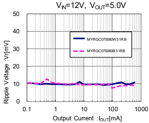
(3) Ripple Voltage vs. Output Current (MYRGC075060W31RB / MYRGC075060B31RB)
