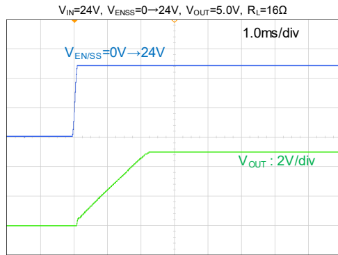
(20) Start-up Waveform ( V_{IN} Rising)
