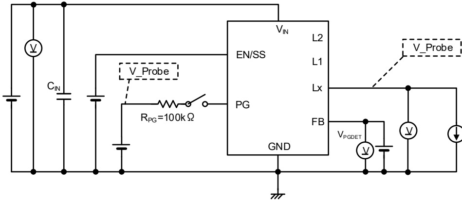
CIRCUIT⑤
