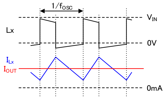
MYRGC075060W31RB (F-PWM control) : Example of heavy load operation
