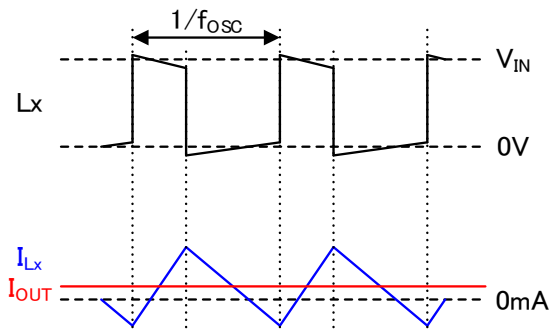
MYRGC075060W31RB (F-PWM control) : Example of light load operation
