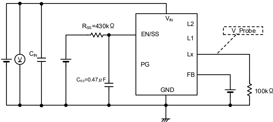
CIRCUIT③
