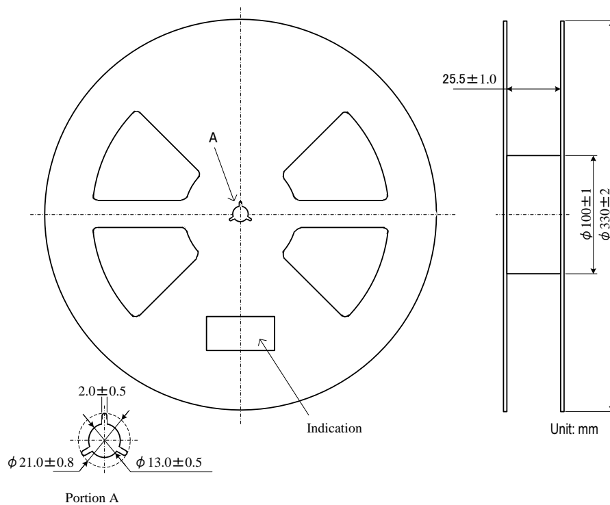
Figure 36. Reel Dimension
