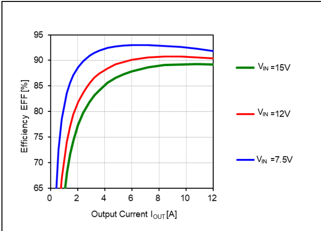
Figure 5. Efficiency vs. Load Current and Line Voltage
