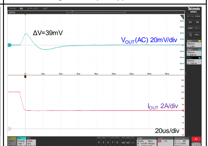
( V_{IN} = 12V, V_{OUT} = 1.8V, C_{OUT} = 600\mu F, I_{OUT} = 12 \text{ to } 6A, 1.2A/\mu s ) Figure 10. Step Load Transient Response
