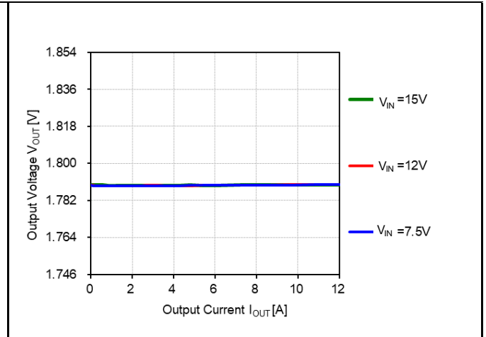
Figure 6. V_{OUT} vs. Load Current and Line Voltage
