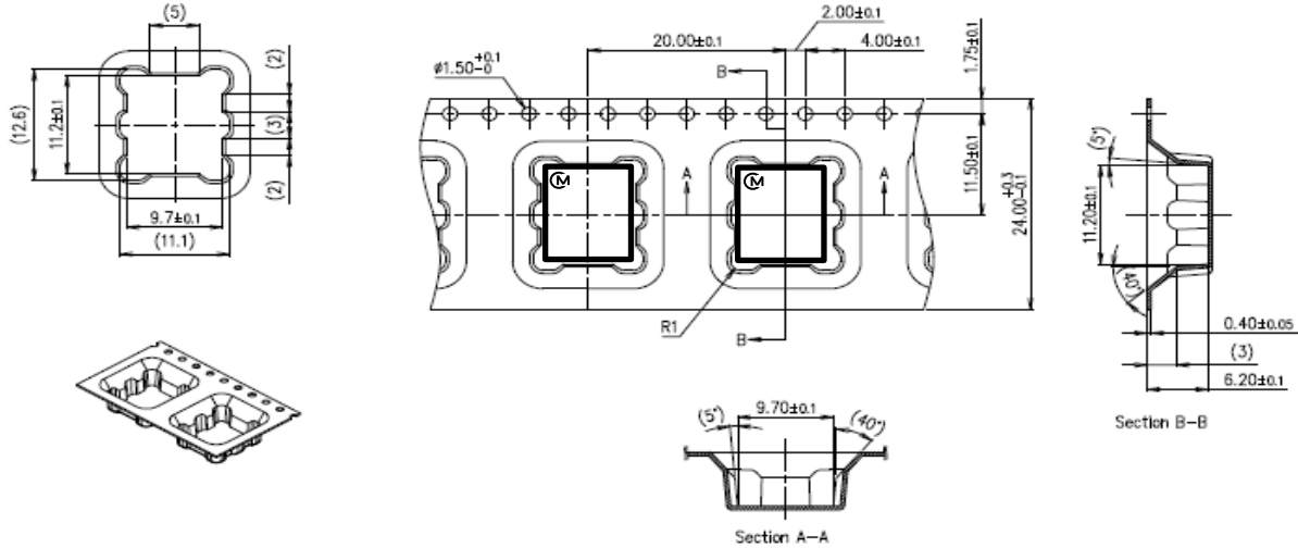
Figure 35. Tape Dimension
