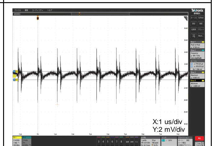
( V_{IN} = 12V, I_{OUT} = 12A, C_{OUT} = 600\mu F, \text{ScopeBW} = 20\text{MHz} ) Figure 8. Output Ripple and Noise
