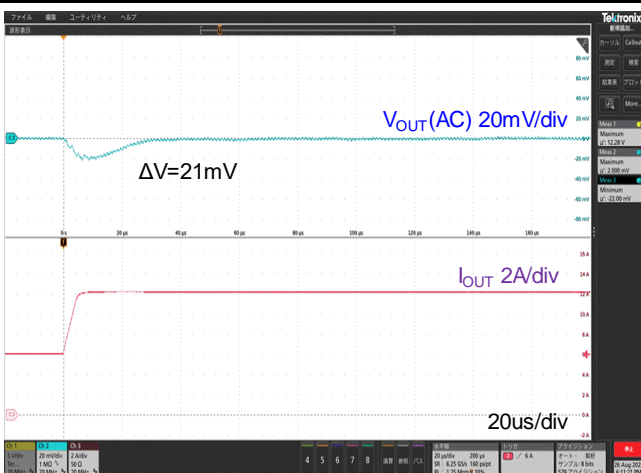
Figure 21. Step Load Transient Response
