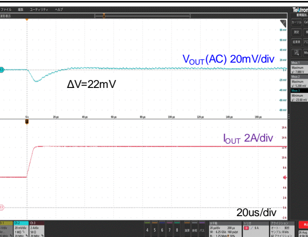
Figure 15. Step Load Transient Response
