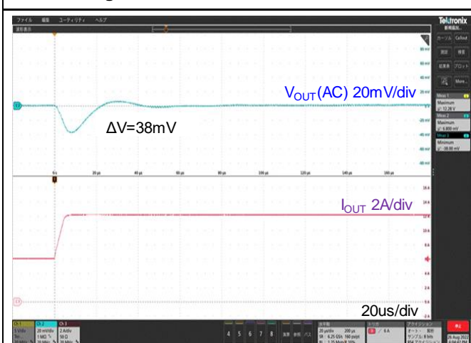
( V_{IN} = 12V, C_{OUT} = 600\mu F, I_{OUT} = 6 \text{ to } 12A, 1.2A/\mu s ) Figure 9. Step Load Transient Response
