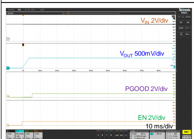
( V_{IN} = 12V, I_{OUT} = 12A ) Figure 7. On/Off Enable Wave Form
