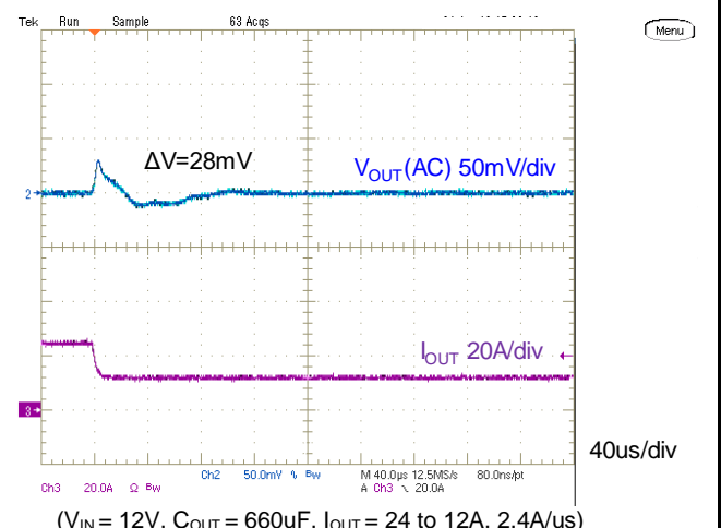
Figure 16. Step Load Transient Response
