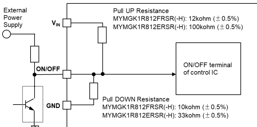
Figure 10. ON/OFF Internal Circuit Diagram
