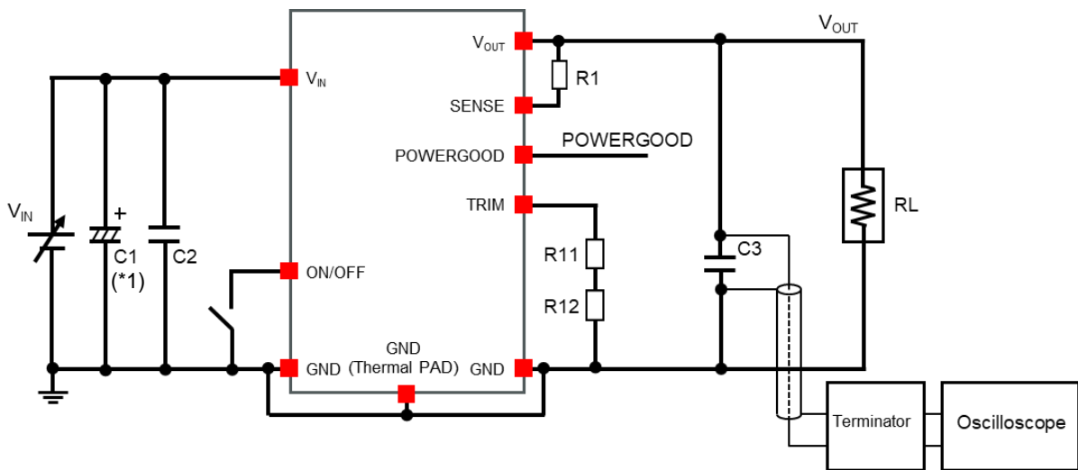
Figure 7. Test Circuit
