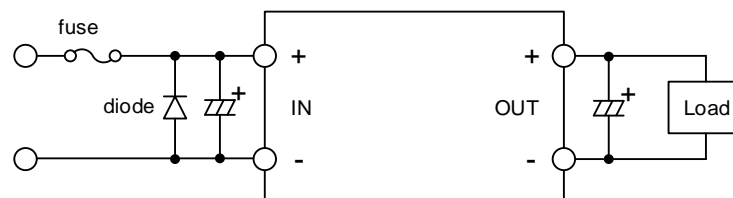
Figure 20. Circuit example with a diode and fuse
