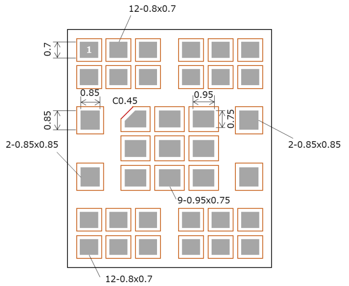
(b) Metal Mask Design
