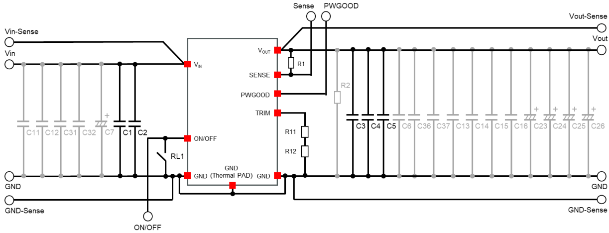
Figure 11. Application Circuit
