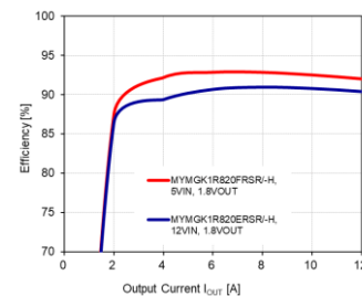
Figure 1. Efficiency Curve
