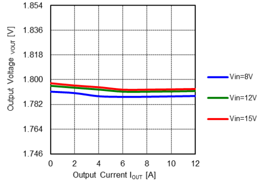
V_{OUT} vs. Load Current
