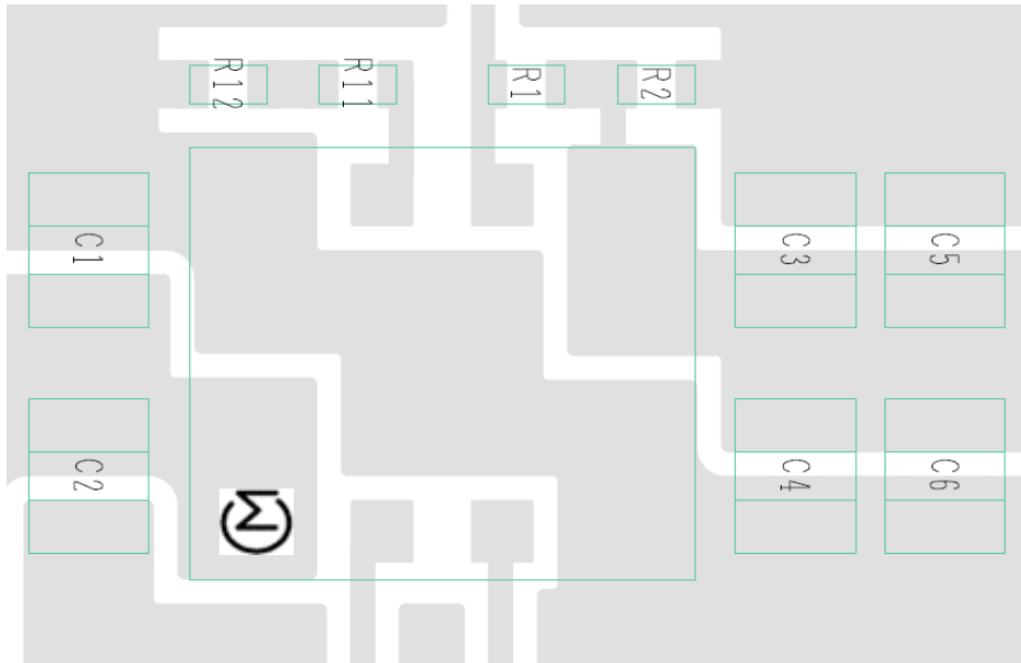
Figure 12. Example of Pattern Layout (Top View)
