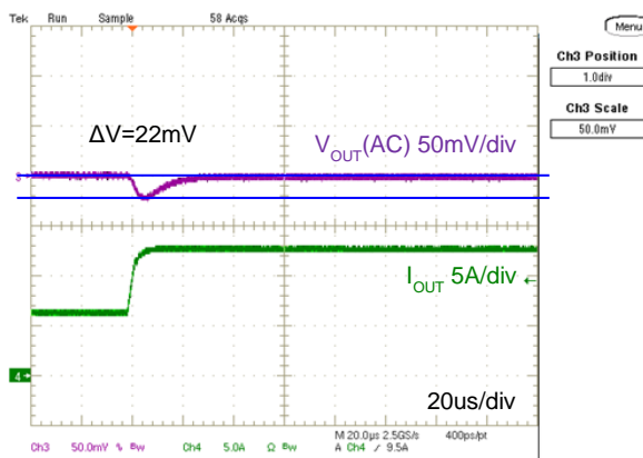
Step Load Transient Response
