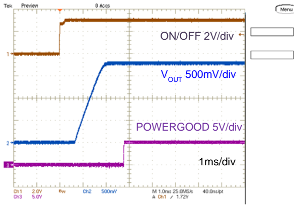
On/Off Enable Waveform ( V_{IN} = 12V, I_{OUT} = 12A )
