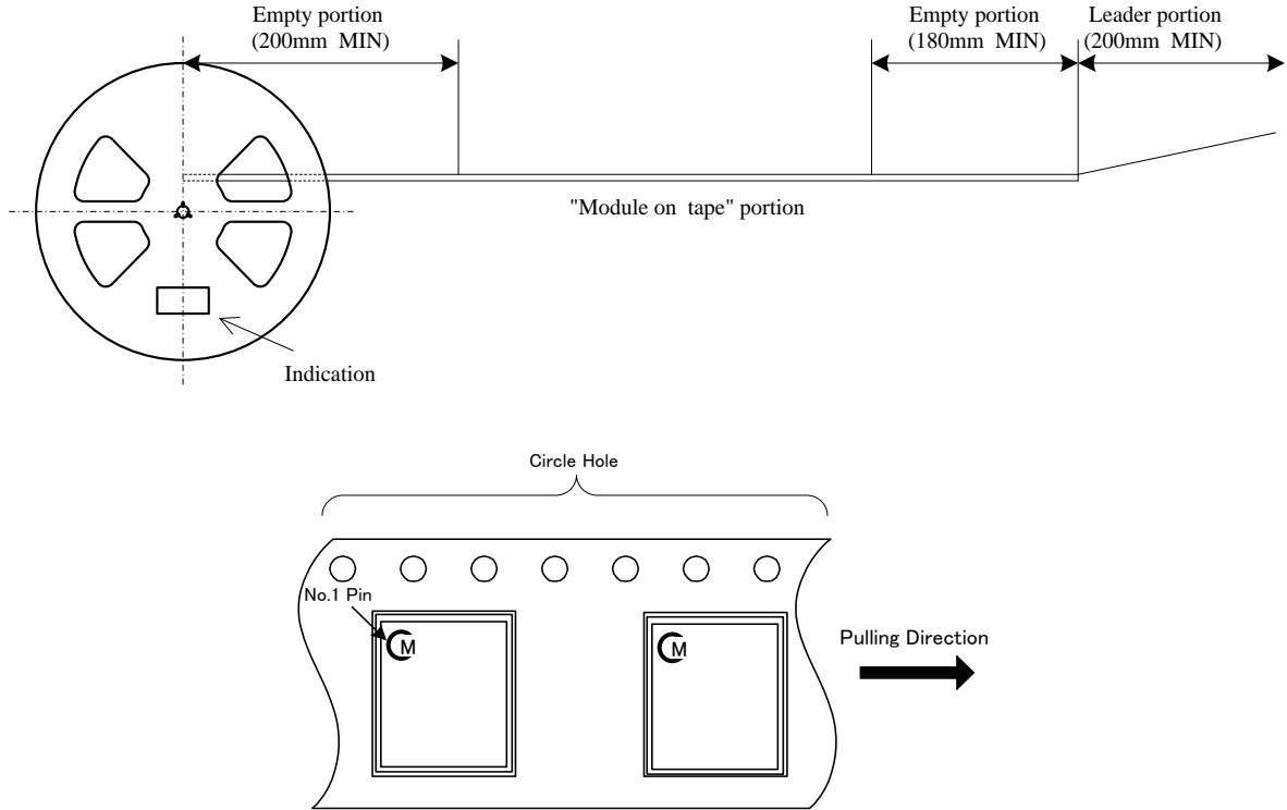
Figure 18. Tape Specifications
