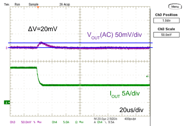
( V_{IN} = 12V, C_{OUT} = 660\mu F, I_{OUT} = 12 \text{ to } 6A, 1.2A/us )
