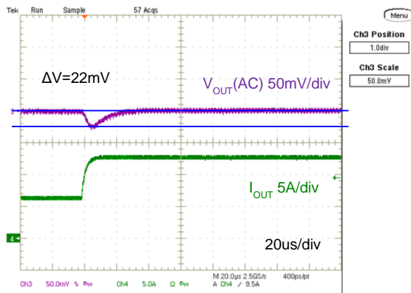
( V_{IN} = 12V, C_{OUT} = 660\mu F, I_{OUT} = 6 \text{ to } 12A, 1.2A/us )
