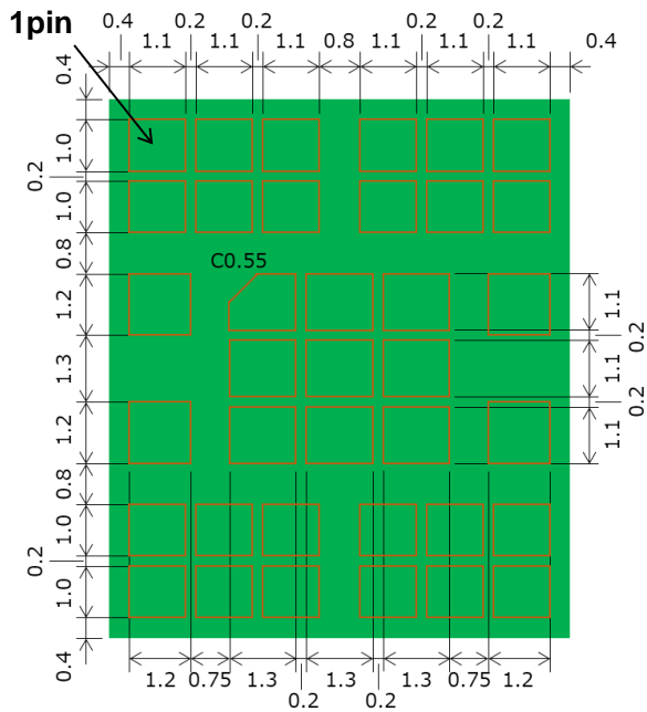
(a) Board Land Pattern
