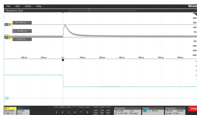
Transient Response (Vin=12V, Vout=5.0V, Cout=400uF, Iout=10 to 5A, 1.0A/us)
