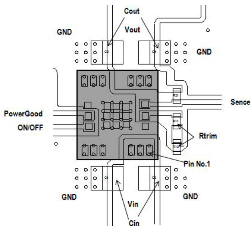
Example of Pattern Layout (Top View)
