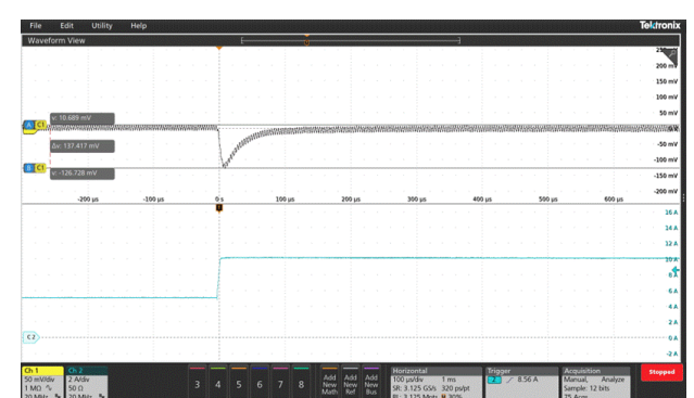
Transient Response (Vin=12V, Vout=5.0V, Cout=400uF, Iout=5 to 10A, 1.0A/us)
