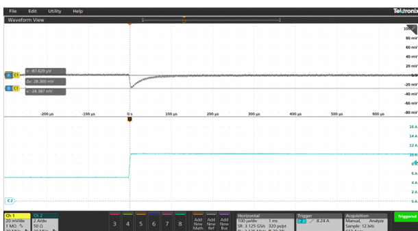
Transient Response (Vin=12V, Vout=1.0V, Cout=400uF, Iout=5 to 10A, 1.0A/us)
