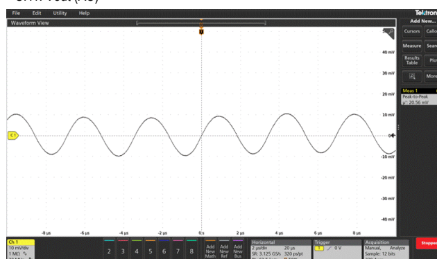
Output Ripple Noise (Vin=12V, Vout=5.0V, Iout=10A, Cout=400uF)
