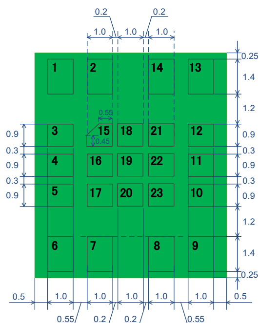
Recommended Board Land Pattern (Top View)
