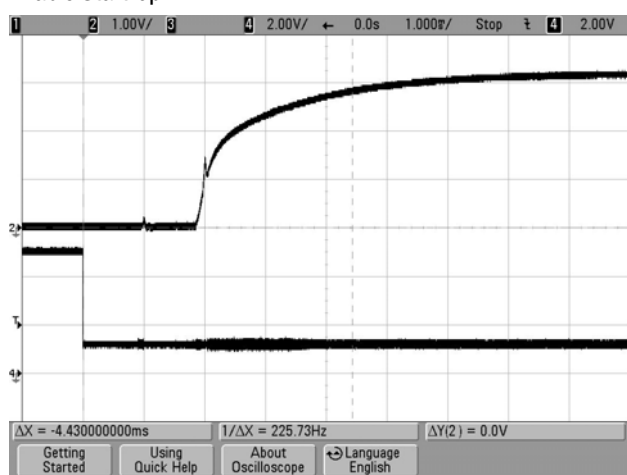
Enable Start-up ( V_{IN}=48V I_{out}=20A )
