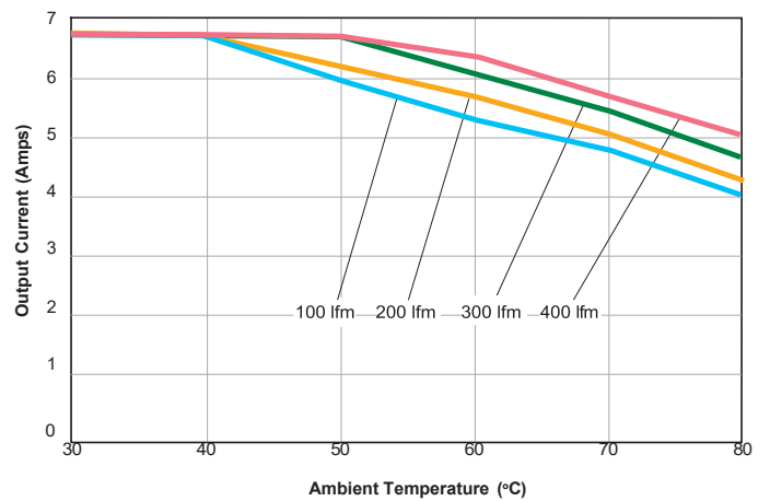
UCH-15/6.7-D48 Maximum Current Temperature Derating (at sea level) No baseplate, V_{IN} = 48V , transverse airflow
