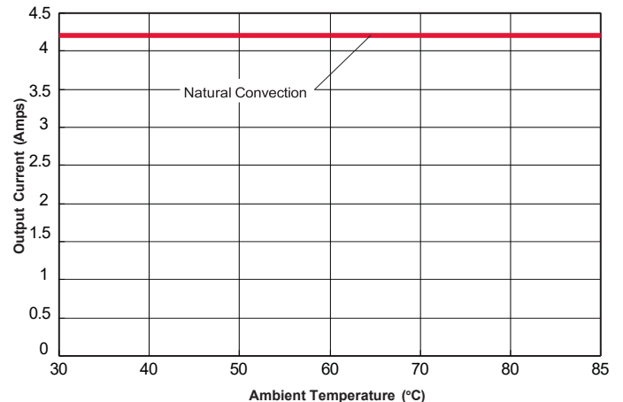
UCH-12/4.2-D48 Maximum Current Temperature Derating at sea level (VIN = 48V, airflow direction from VIN to VOUT, no baseplate)
