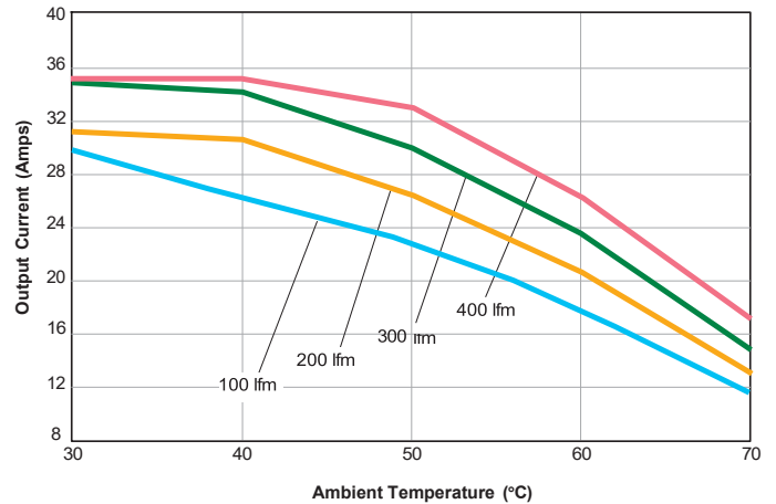
UCH-3.3/35-D24 Maximum Current Temperature Derating (at sea level) No baseplate, V_{IN} = 24V , transverse airflow
