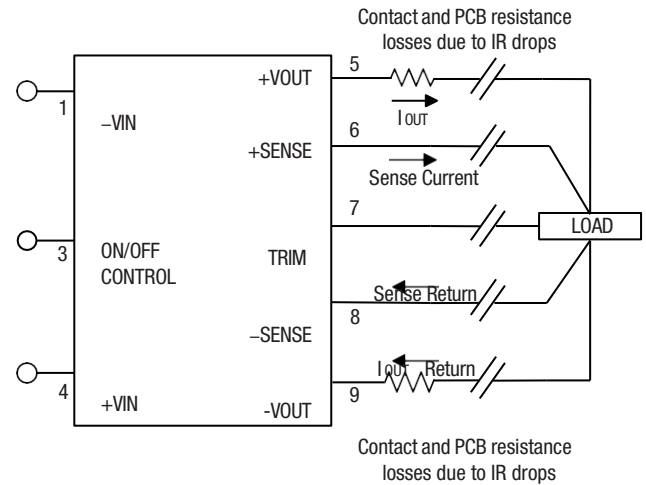
Figure 4. Remote Sense Circuit Configuration
