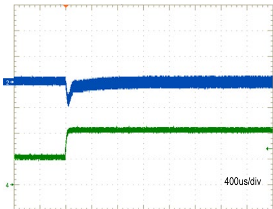
Transient Response ( V_{IN} = 48V , I_{OUT} = 1.06 to 2.125A , T_a = 25\text{degC} ) Ch2 = V_{OUT} , 200mV/div, Ch4 = I_{OUT} , 1A/div
