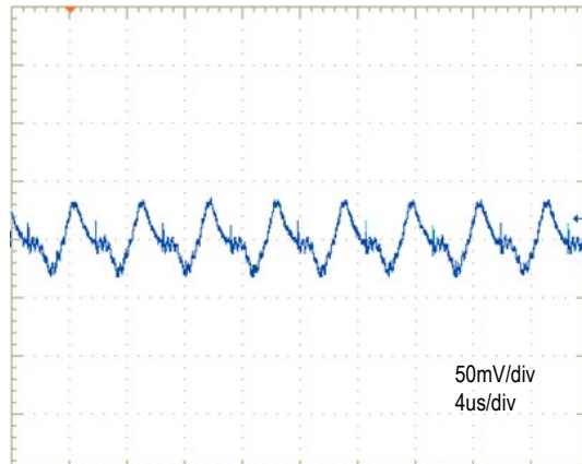
Output Ripple and Noise ( V_{IN} = 48V , I_{OUT} = 2.125A , T_a = 25\text{degC} )
