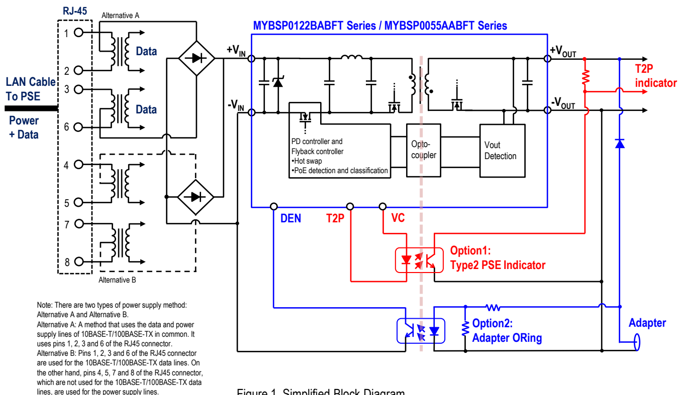
Figure 1. Simplified Block Diagram Typical topology is shown.
