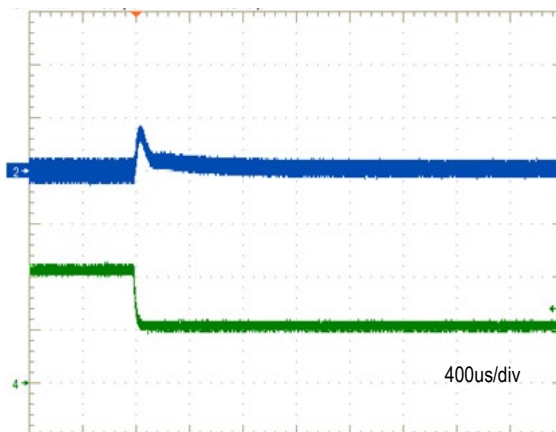
Transient Response ( V_{IN} = 48V , I_{OUT} = 2.125 to 1.06A , T_a = 25\text{degC} ) Ch2 = V_{OUT} , 200mV/div, Ch4 = I_{OUT} , 1A/div
