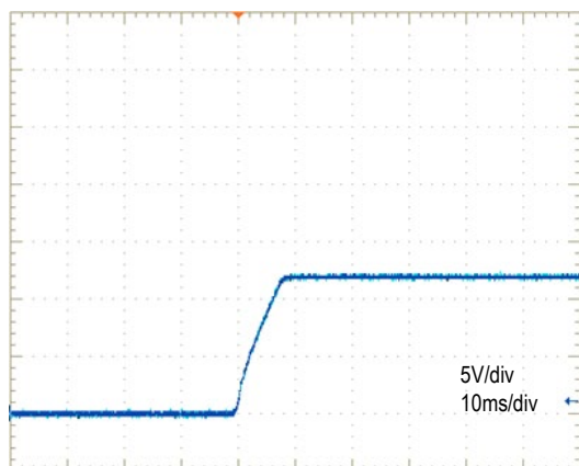
V_{OUT} Start-up ( V_{IN} = 48V , I_{OUT} = 2.125A , T_a = 25\text{degC} )
