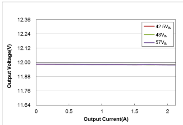
Load Regulation ( T_a = 25\text{degC} )
