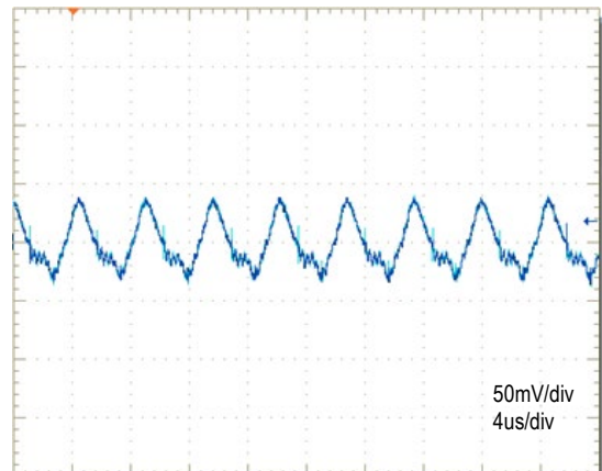
Output Ripple and Noise ( V_{IN} = 48\text{V} , I_{OUT} = 5.1\text{A} , T_a = +25\text{degC} )
