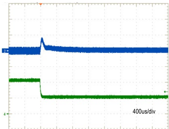
Transient Response ( V_{IN} = 48\text{V} , I_{OUT} = 2.125 to 1.06\text{A} , T_a = +25\text{degC} ) Ch2 = V_{OUT} , 200mV/div, Ch4 = I_{OUT} , 1A/div
