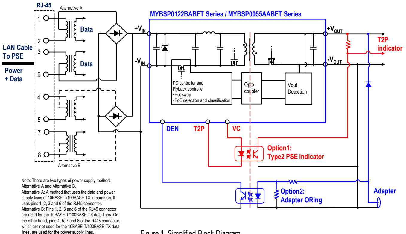
Figure 1. Simplified Block Diagram Typical topology is shown.
