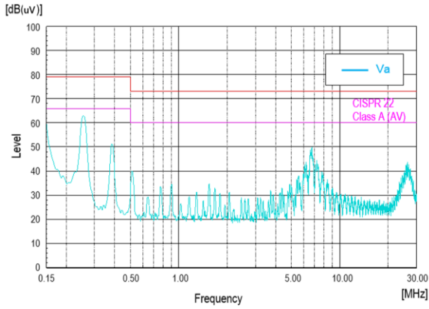
Conduction Noise ( V_{IN} = 48V, I_{OUT} = 1A, T_a = +25degC ) with External Input Filter
