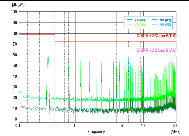
( V_{IN} = 48V , I_{OUT} = 4.25A , T_a = 25degC ) with External Input Filter Figure 9. Conduction Noise
