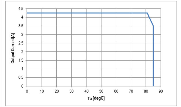
Unit under test (UUT) is covered by acrylic box to avoid airflow. ( V_{IN} = 48V , See Technical Notes ) Figure 11. Thermal Derating
