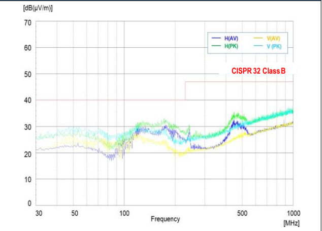
( V_{IN} = 48V , I_{OUT} = 4.25A , T_a = 25degC ) with External Input Filter Figure 10. Radiation Noise
