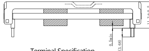
Terminal Specification Sn(100%), Ni over Copper Base
