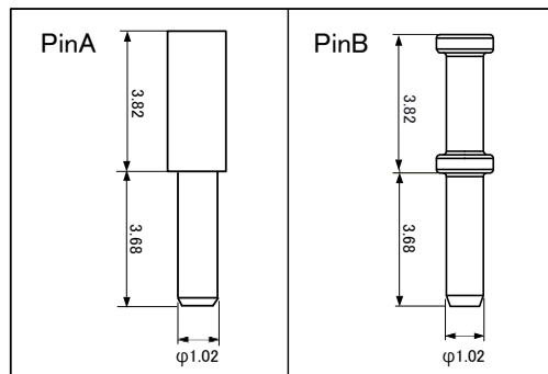
*Pins 1, 2, 3, 5, 6 and 7 use either Pin A or Pin B.
