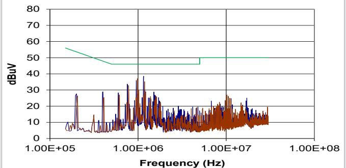
NCM3S1205MC (Average)
