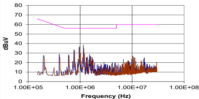
NCM3S1205MC (Quasi-Peak)
