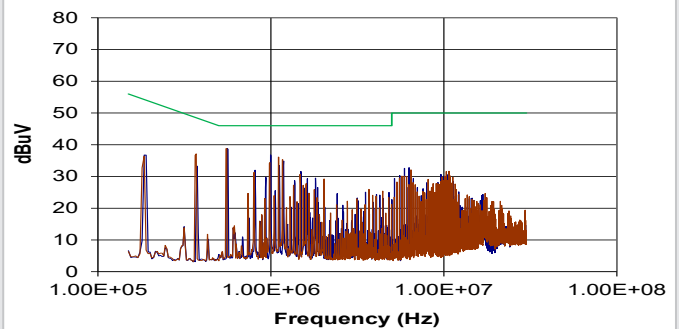
NCM3S1212MC (Average)
