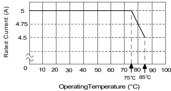
DLW5BSM191SQ2 Temperature Derating
