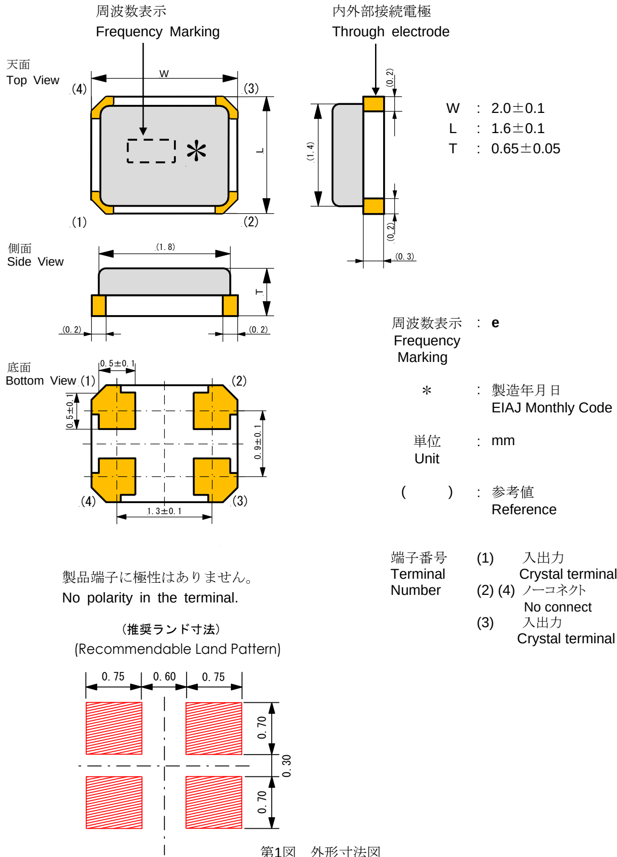
Figure 1. Dimensions
