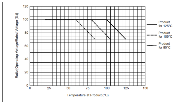
Recommended derating conditions on voltage and temperature
