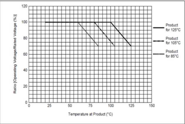
Derating conditions on Voltage and Temperature (for Rated Voltage 100Vdc max.)
