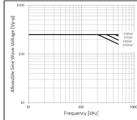
Chip(L×W): 2.0×1.25mm C0G(5C) Char. Rated Voltage:DC250V
