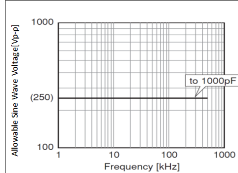
Chip(L×W): 1.0×0.5mm 1.6×0.8mm C0G(5C) Char. Rated Voltage:DC250V
