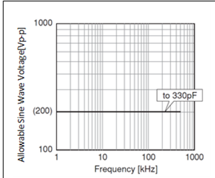
Chip(L×W): 2.0×1.25mm C0G(5C) Char. Rated Voltage:DC200V
