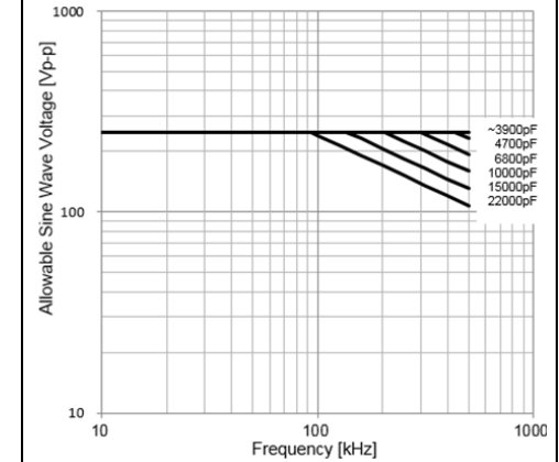
Chip(L×W): 3.2×1.6mm C0G(5C) Char. Rated Voltage:DC250V
