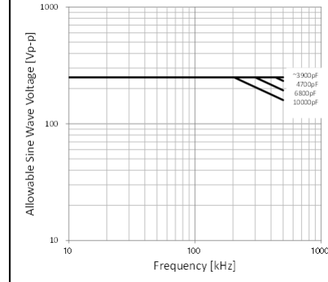
Chip(L×W): 2.0×1.25mm C0G(5C) Char. Rated Voltage:DC250V
