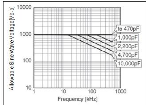
Chip(L×W): 3.2×1.6mm/3.2×2.5mm/ 4.5×3.2mm/5.7×5.0mm U2J(7U) Char. Rated Voltage:DC1 kV
