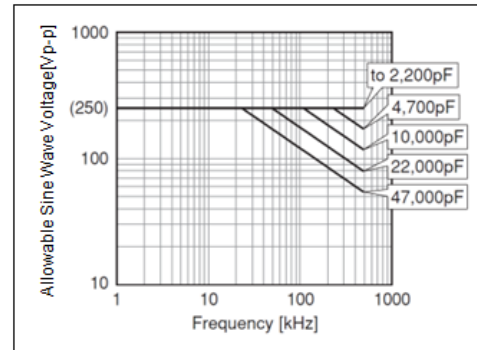
Chip(L×W): 2.0×1.25mm/3.2×1.6mm U2J(7U) Char. Rated Voltage:DC250V
