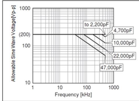
Chip(L×W): 2.0×1.25mm/3.2×1.6mm U2J(7U) Char. Rated Voltage:DC200V
