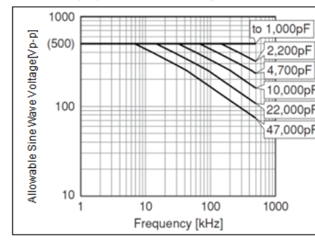
Chip(L×W): 3.2×1.6mm/3.2×2.5mm/ 4.5×3.2mm/5.7×5.0mm U2J(7U) Char. Rated Voltage:DC500V
