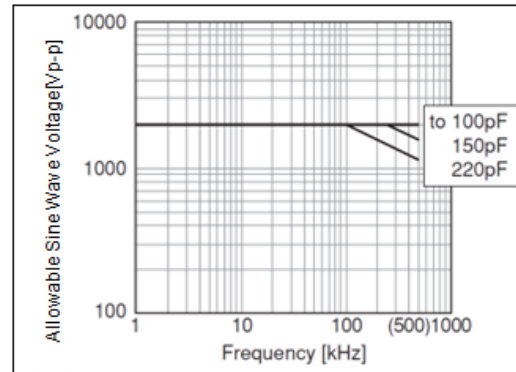
Chip(L×W): 3.2×1.6mm/3.2×2.5mm U2J(7U) Char. Rated Voltage:DC2 kV
