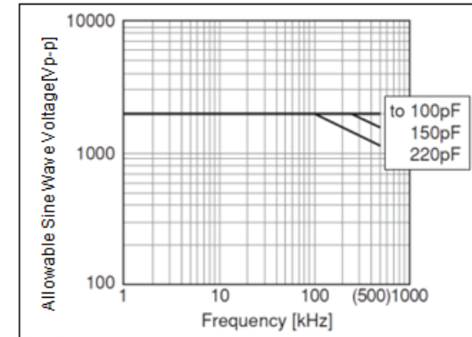
Chip(L×W): 4.5×2.0mm U2J(7U) Char. Rated Voltage:DC3.15kV
