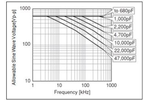
Chip(L×W): 3.2×1.6mm/3.2×2.5mm/ 4.5×3.2mm/5.7×5.0mm U2J(7U) Char. Rated Voltage:DC630V
