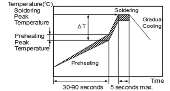
[ Allowable Flow Soldering Temperature and Time ]
