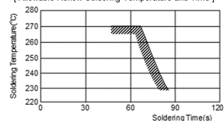
[ Allowable Reflow Soldering Temperature and Time ]
