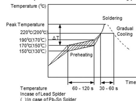
[ Allowable Reflow Soldering Temperature and Time ]
