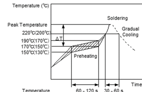
[ Standard Conditions for Reflow Soldering ]
