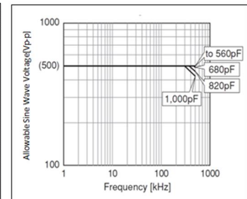
Chip(LxW): 3.2x1.6mm C0G(5C) Char. Rated Voltage:DC500V
