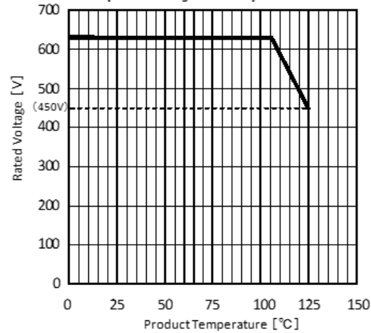
Fig:Derating
