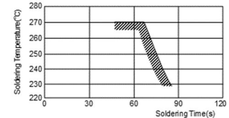
[ Allowable Reflow Soldering Temperature and Time ]
