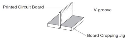
[Outline of Jig]
